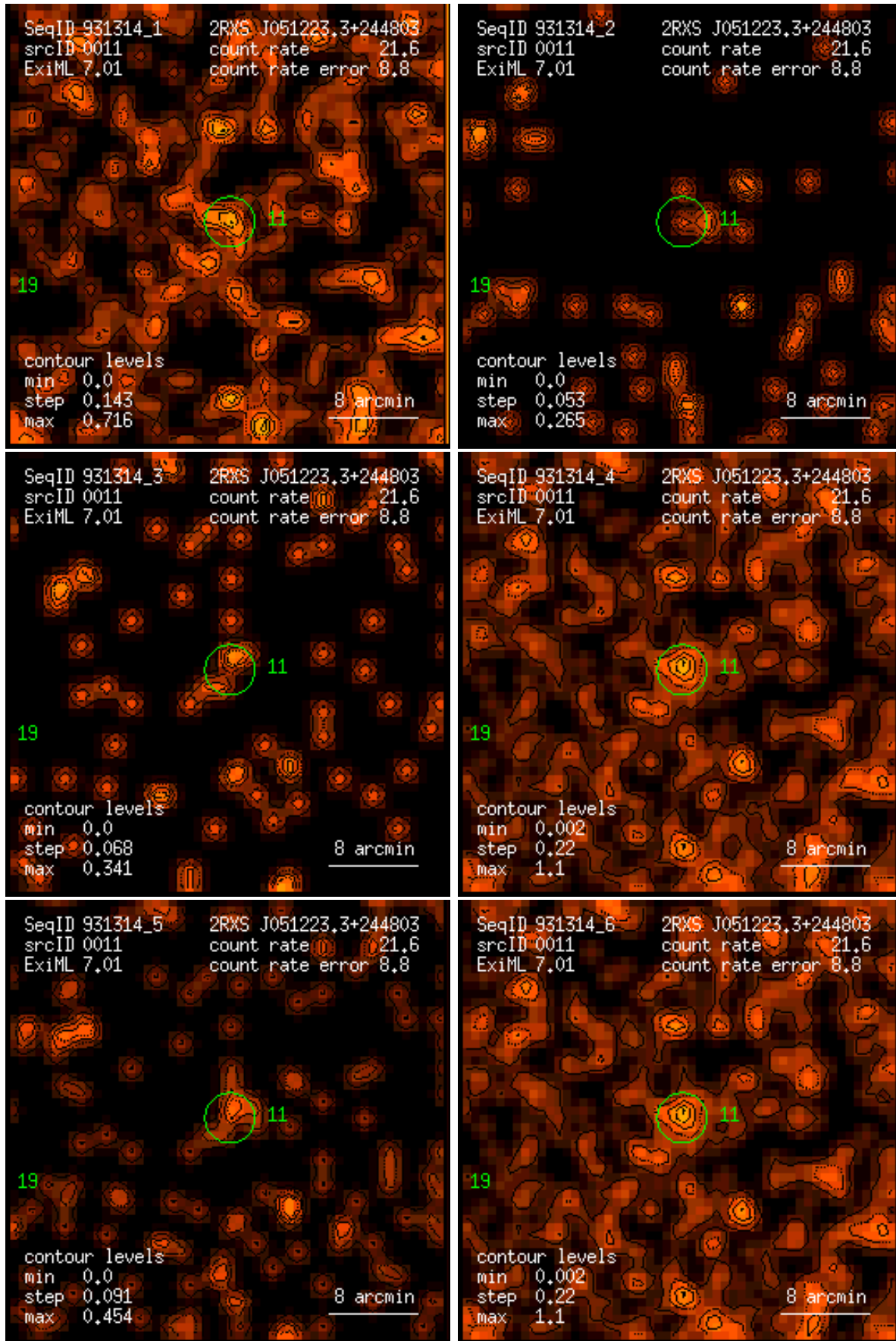
Figure 11: RASS 931314: detection 0011: band rate images, Gaussian filter: (1) PSPC channels 11 – 41, (2) 52 – 90, (3) 91 – 201, (4) 11 – 235, (5) 52 – 201, (6) 11 – 201. Broad band rates in counts/ks. Band rate contour levels in counts/ks/arcmin 2 .
