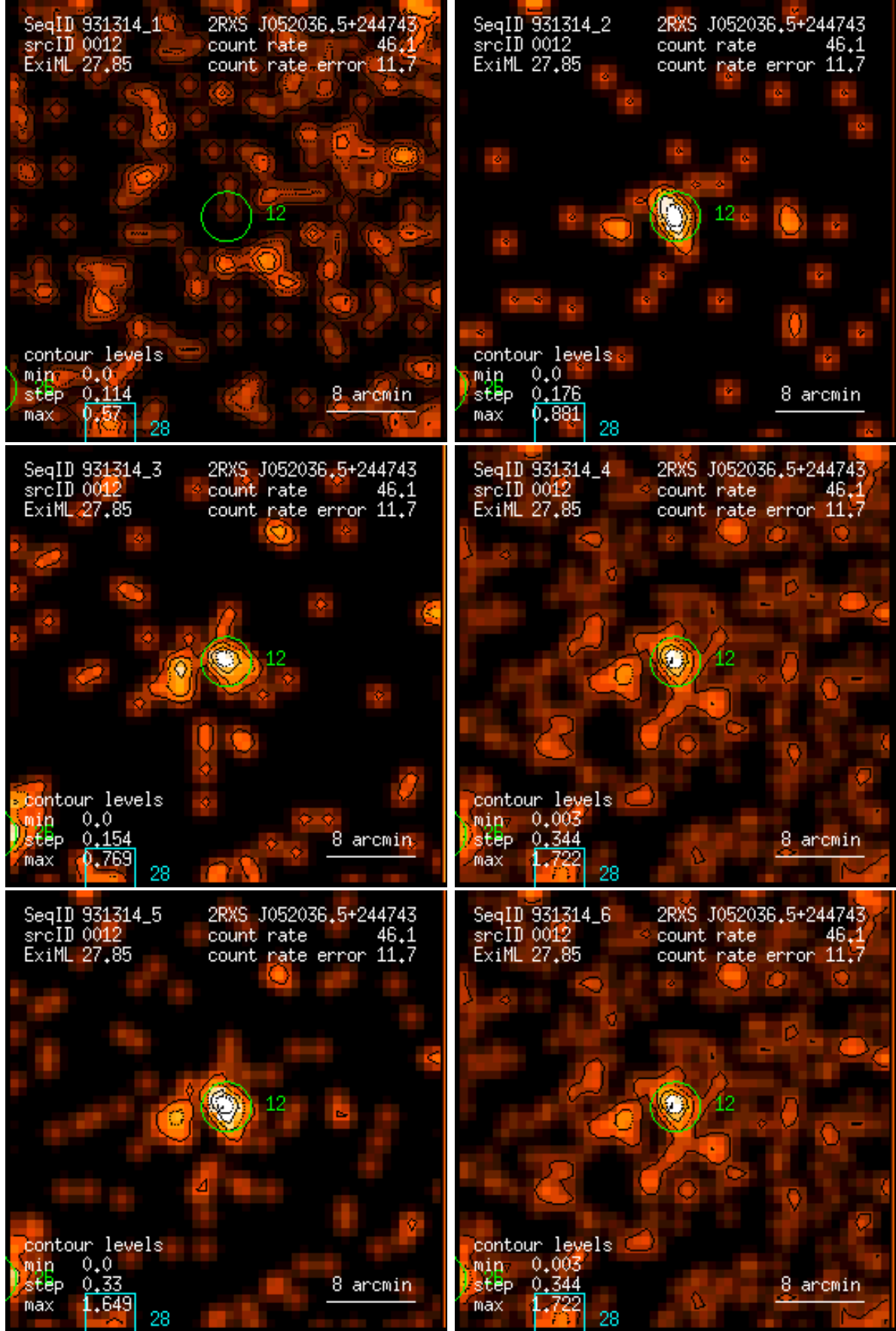
Figure 12: RASS 931314: detection 0012: band rate images, Gaussian filter: (1) PSPC channels 11 – 41, (2) 52 – 90, (3) 91 – 201, (4) 11 – 235, (5) 52 – 201, (6) 11 – 201. Broad band rates in counts/ks. Band rate contour levels in counts/ks/arcmin 2 .
