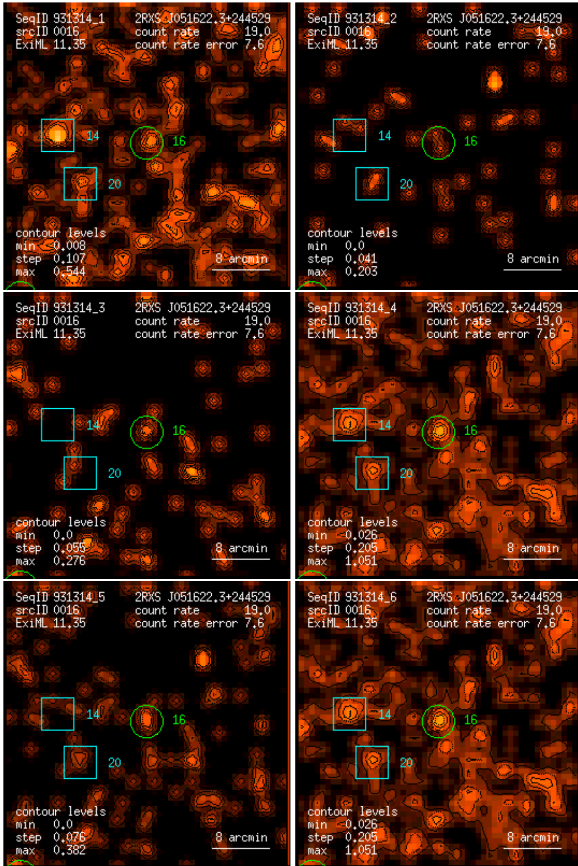
Figure 16: RASS 931314: detection 0016: band rate images, Gaussian filter: (1) PSPC channels 11 – 41, (2) 52 – 90, (3) 91 – 201, (4) 11 – 235, (5) 52 – 201, (6) 11 – 201. Broad band rates in counts/ks. Band rate contour levels in counts/ks/arcmin 2 .
