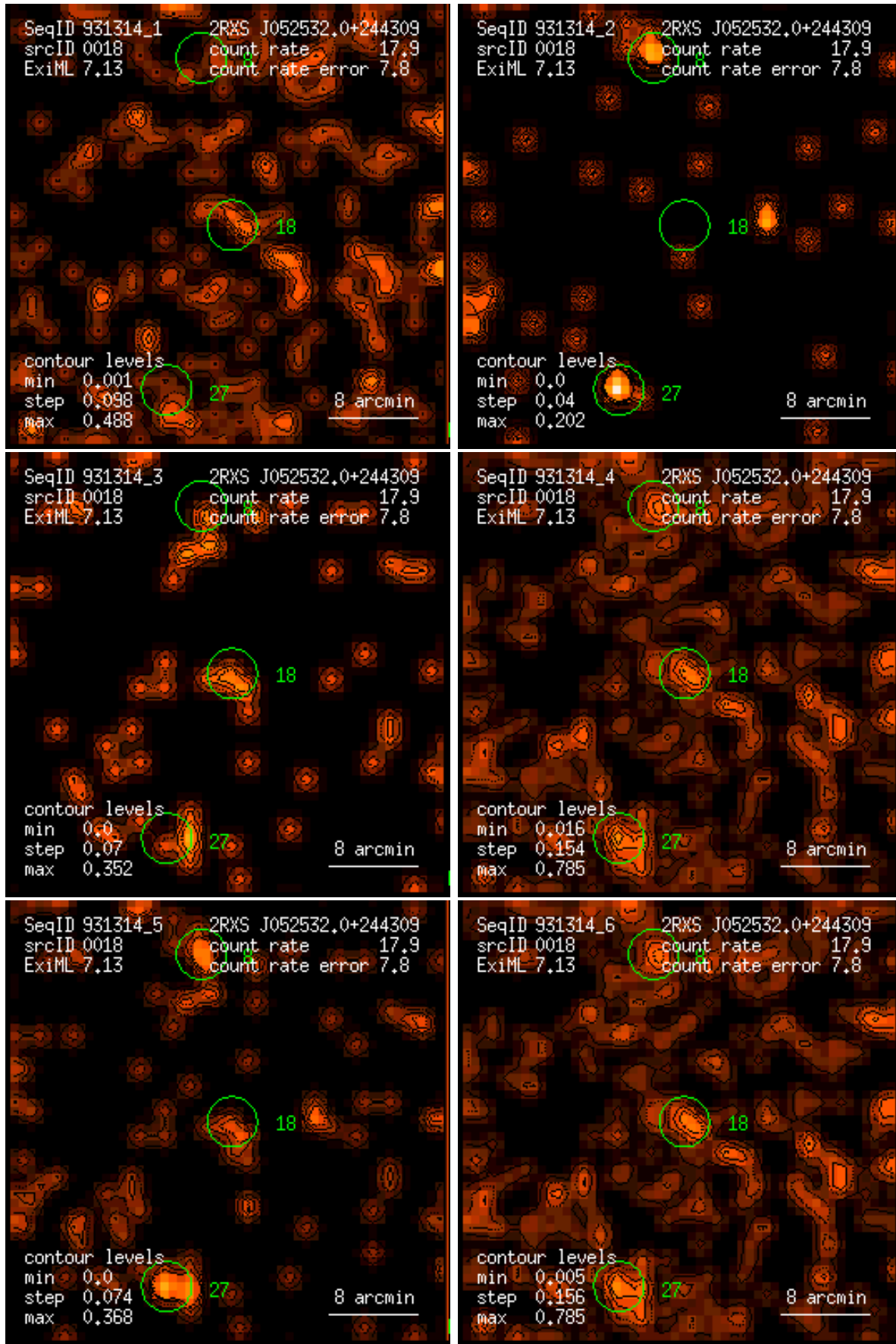
Figure 18: RASS 931314: detection 0018: band rate images, Gaussian filter: (1) PSPC channels 11 – 41, (2) 52 – 90, (3) 91 – 201, (4) 11 – 235, (5) 52 – 201, (6) 11 – 201. Broad band rates in counts/ks. Band rate contour levels in counts/ks/arcmin 2 .
