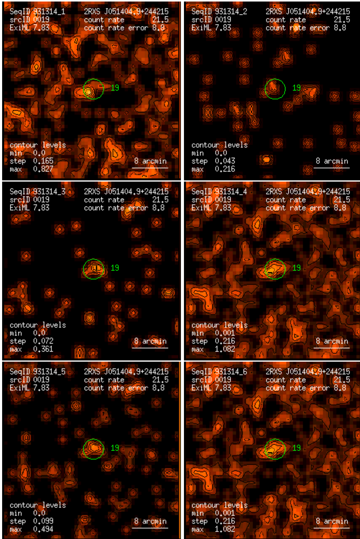
Figure 19: RASS 931314: detection 0019: band rate images, Gaussian filter: (1) PSPC channels 11 – 41, (2) 52 – 90, (3) 91 – 201, (4) 11 – 235, (5) 52 – 201, (6) 11 – 201. Broad band rates in counts/ks. Band rate contour levels in counts/ks/arcmin 2 .
