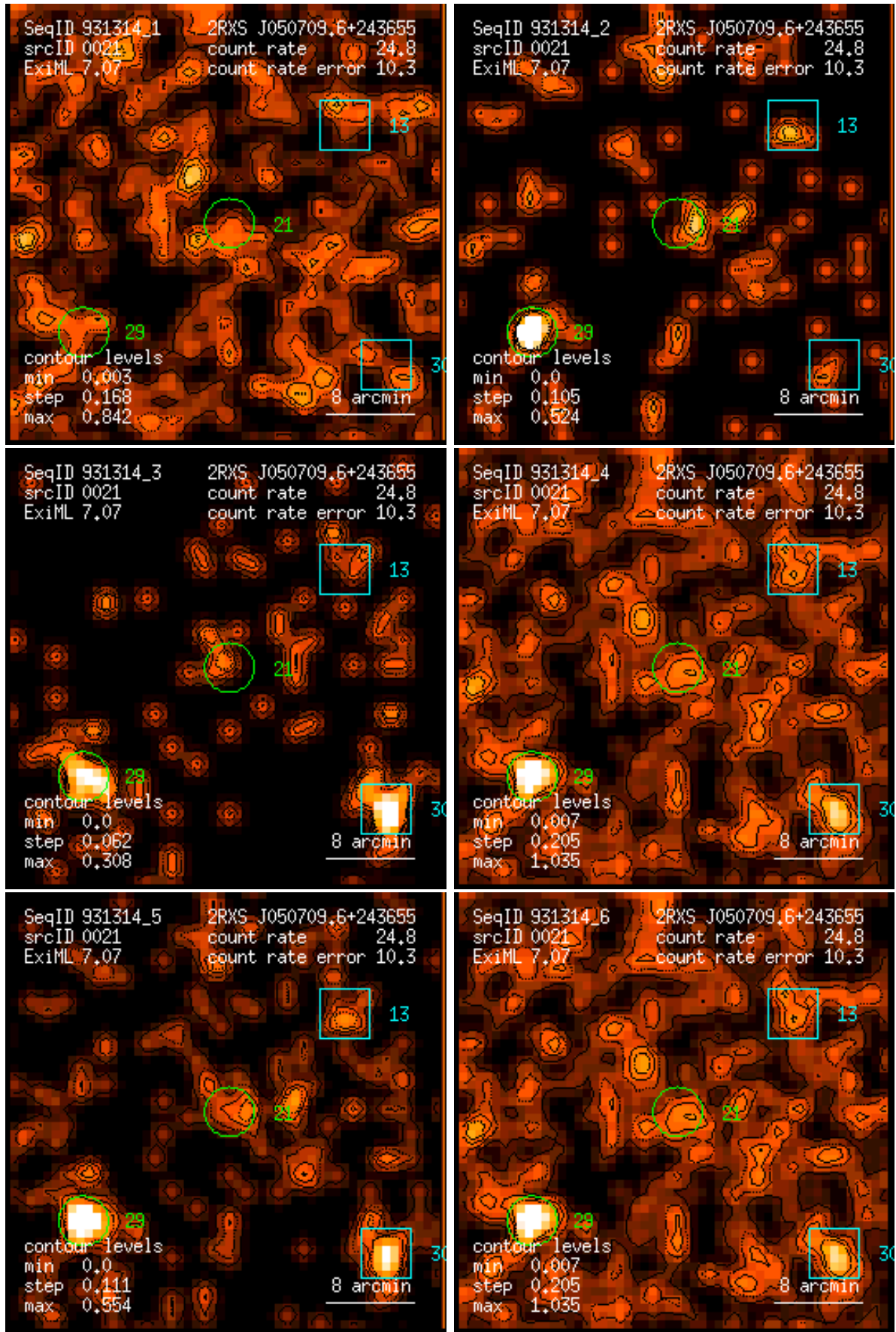
Figure 21: RASS 931314: detection 0021: band rate images, Gaussian filter: (1) PSPC channels 11 – 41, (2) 52 – 90, (3) 91 – 201, (4) 11 – 235, (5) 52 – 201, (6) 11 – 201. Broad band rates in counts/ks. Band rate contour levels in counts/ks/arcmin 2 .
