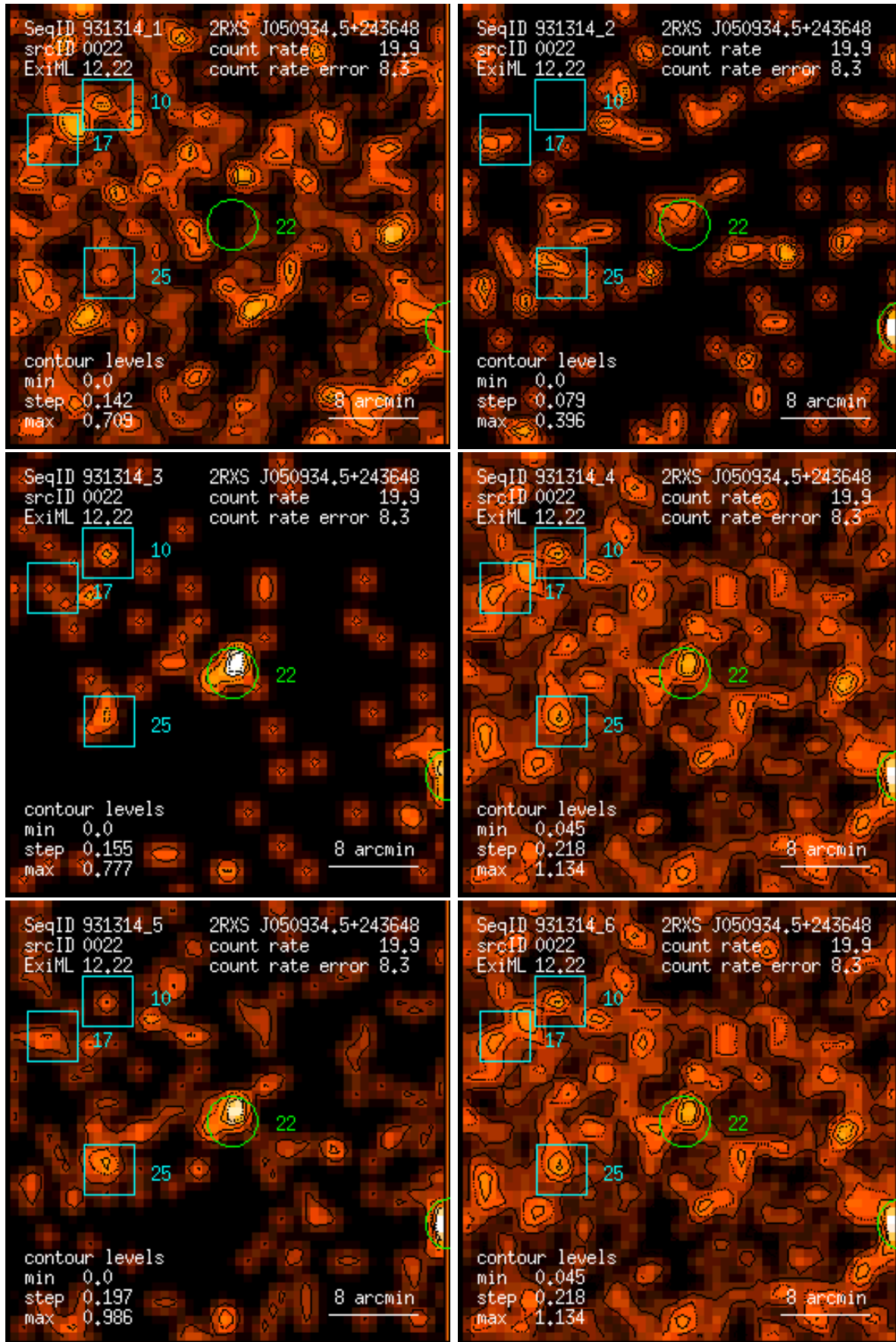
Figure 22: RASS 931314: detection 0022: band rate images, Gaussian filter: (1) PSPC channels 11 – 41, (2) 52 – 90, (3) 91 – 201, (4) 11 – 235, (5) 52 – 201, (6) 11 – 201. Broad band rates in counts/ks. Band rate contour levels in counts/ks/arcmin 2 .
