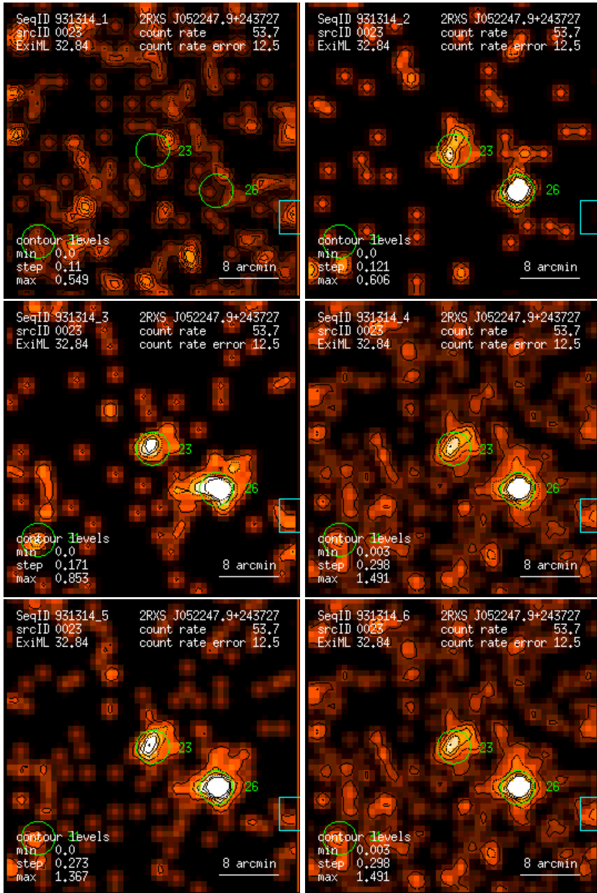
Figure 23: RASS 931314: detection 0023: band rate images, Gaussian filter: (1) PSPC channels 11 – 41, (2) 52 – 90, (3) 91 – 201, (4) 11 – 235, (5) 52 – 201, (6) 11 – 201. Broad band rates in counts/ks. Band rate contour levels in counts/ks/arcmin 2 .
