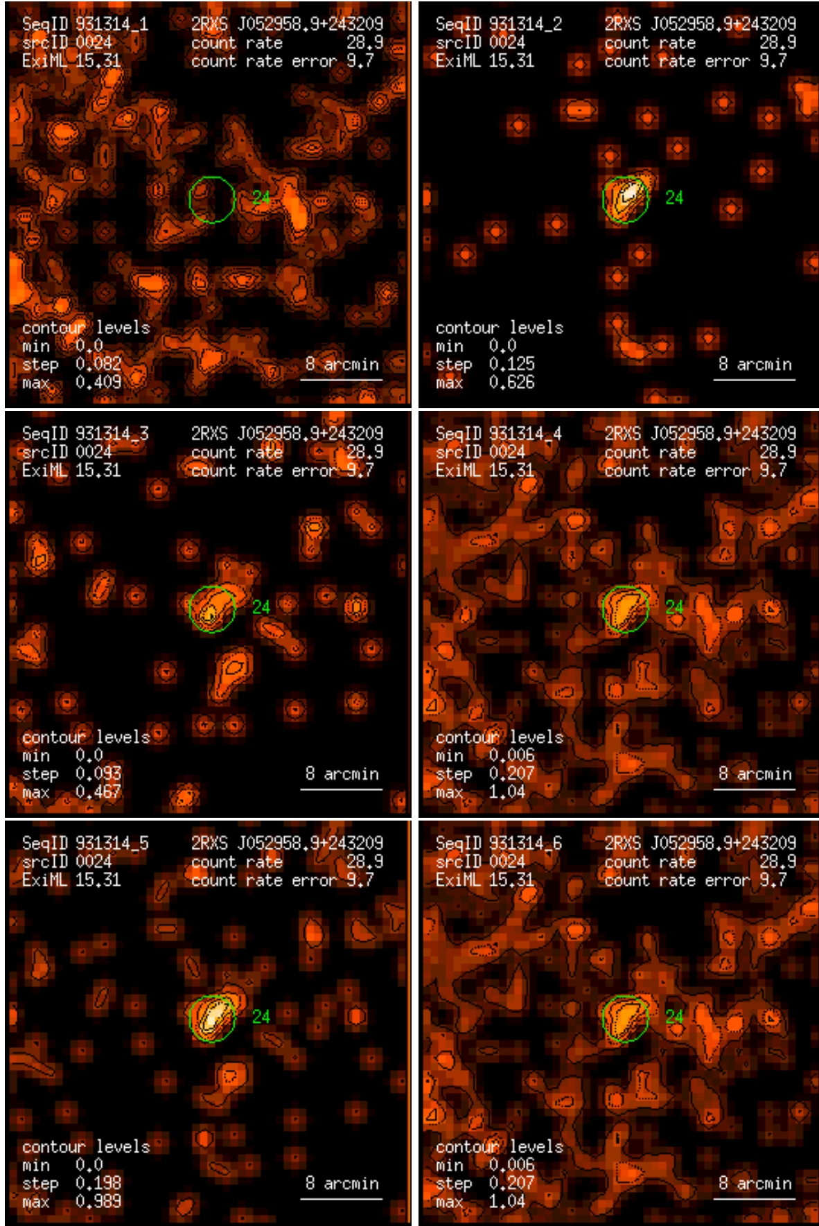
Figure 24: RASS 931314: detection 0024: band rate images, Gaussian filter: (1) PSPC channels 11 – 41, (2) 52 – 90, (3) 91 – 201, (4) 11 – 235, (5) 52 – 201, (6) 11 – 201. Broad band rates in counts/ks. Band rate contour levels in counts/ks/arcmin 2 .
