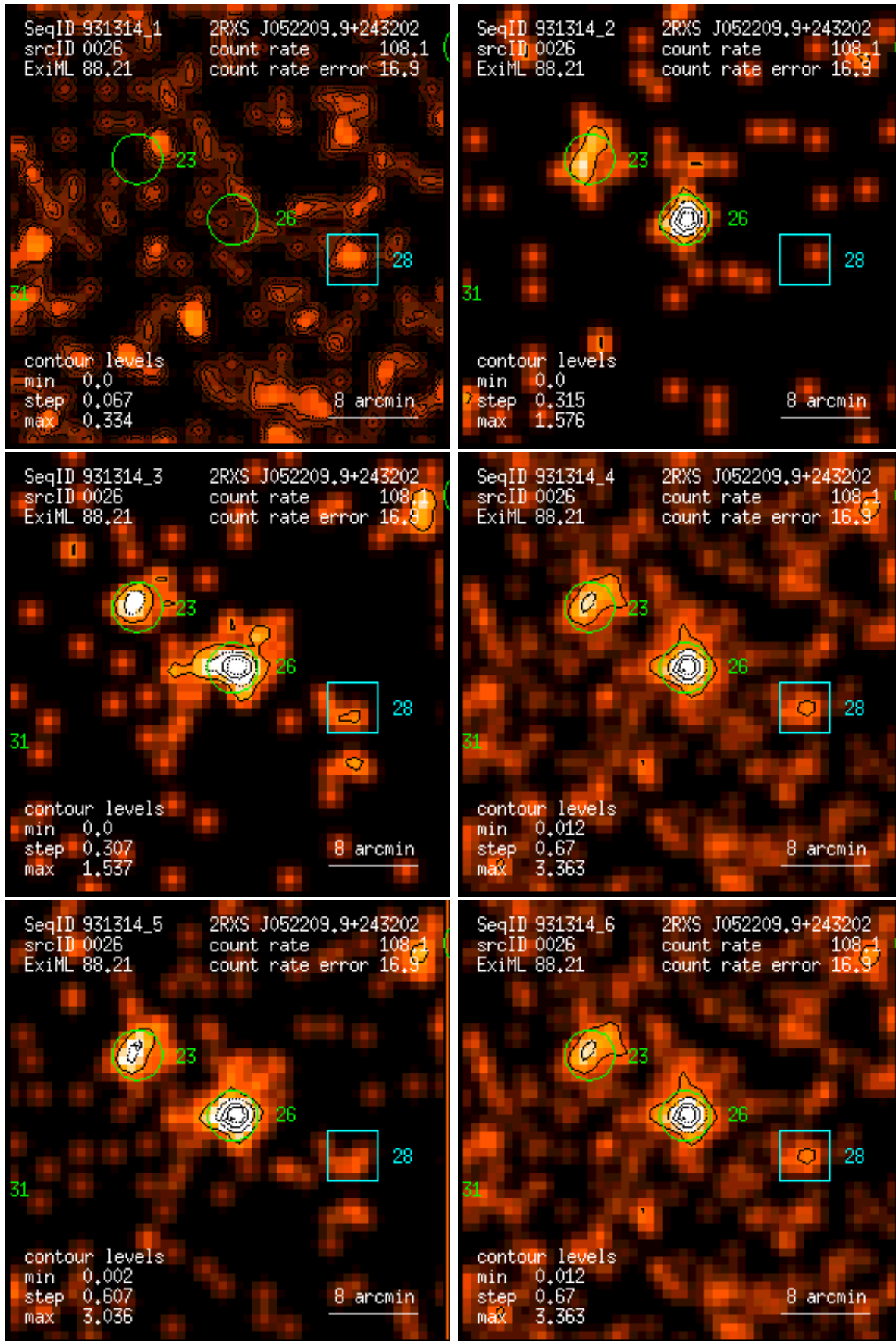
Figure 26: RASS 931314: detection 0026: band rate images, Gaussian filter: (1) PSPC channels 11 – 41, (2) 52 – 90, (3) 91 – 201, (4) 11 – 235, (5) 52 – 201, (6) 11 – 201. Broad band rates in counts/ks. Band rate contour levels in counts/ks/arcmin 2 .
