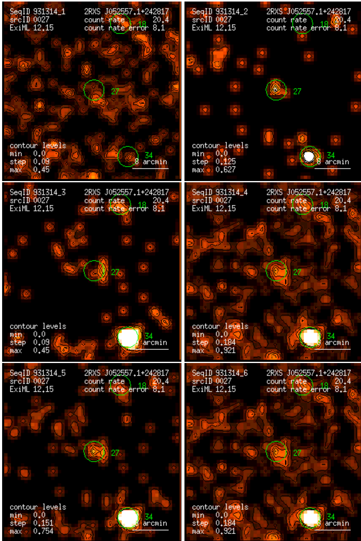
Figure 27: RASS 931314: detection 0027: band rate images, Gaussian filter: (1) PSPC channels 11 – 41, (2) 52 – 90, (3) 91 – 201, (4) 11 – 235, (5) 52 – 201, (6) 11 – 201. Broad band rates in counts/ks. Band rate contour levels in counts/ks/arcmin 2 .
