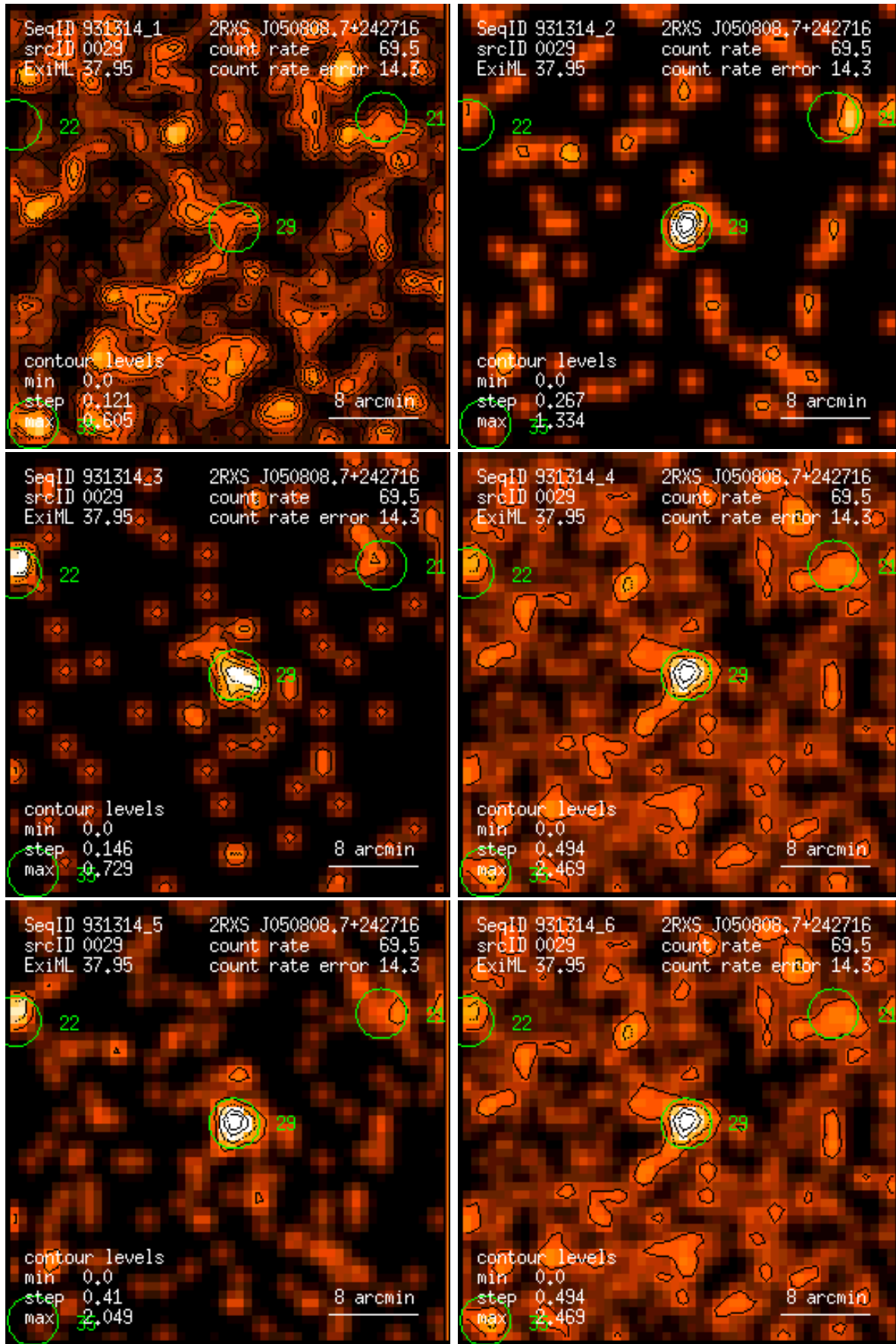
Figure 29: RASS 931314: detection 0029: band rate images, Gaussian filter: (1) PSPC channels 11 – 41, (2) 52 – 90, (3) 91 – 201, (4) 11 – 235, (5) 52 – 201, (6) 11 – 201. Broad band rates in counts/ks. Band rate contour levels in counts/ks/arcmin 2 .
