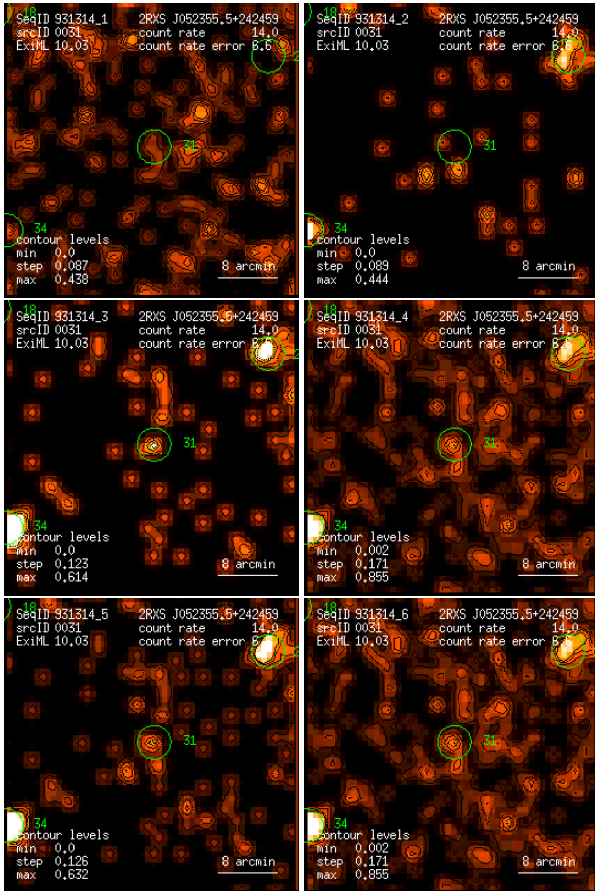
Figure 31: RASS 931314: detection 0031: band rate images, Gaussian filter: (1) PSPC channels 11 – 41, (2) 52 – 90, (3) 91 – 201, (4) 11 – 235, (5) 52 – 201, (6) 11 – 201. Broad band rates in counts/ks. Band rate contour levels in counts/ks/arcmin 2 .
