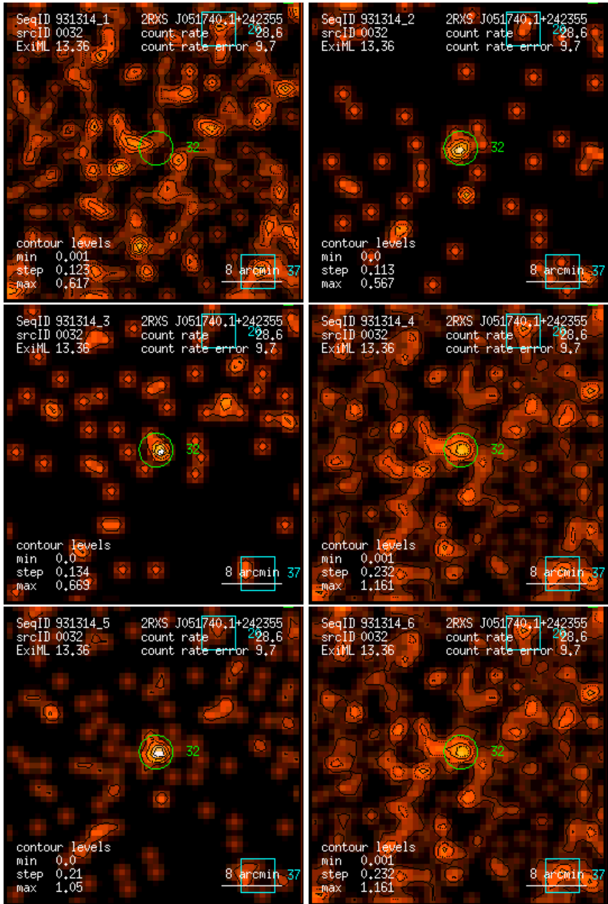
Figure 32: RASS 931314: detection 0032: band rate images, Gaussian filter: (1) PSPC channels 11 – 41, (2) 52 – 90, (3) 91 – 201, (4) 11 – 235, (5) 52 – 201, (6) 11 – 201. Broad band rates in counts/ks. Band rate contour levels in counts/ks/arcmin 2 .
