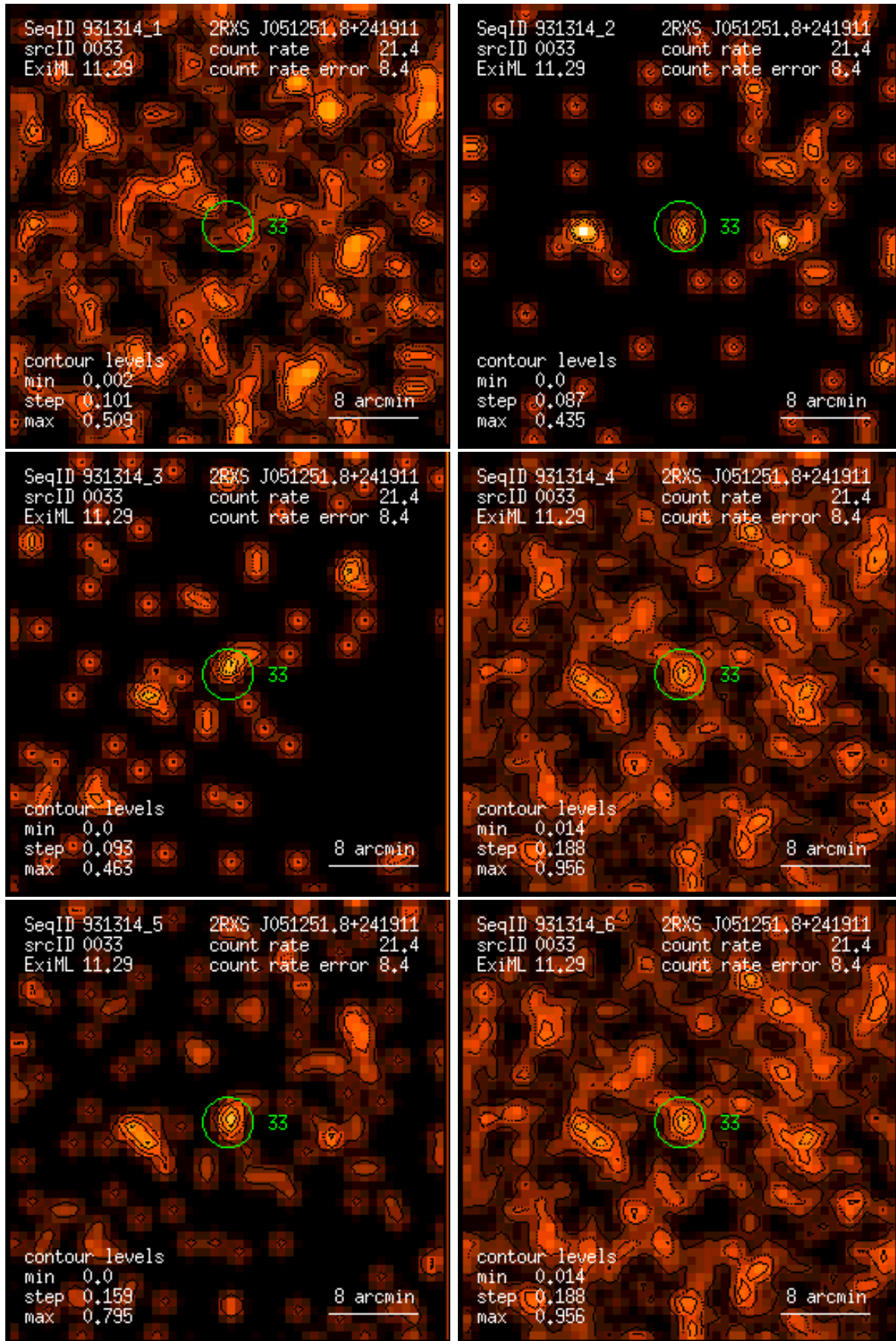
Figure 33: RASS 931314: detection 0033: band rate images, Gaussian filter: (1) PSPC channels 11 – 41, (2) 52 – 90, (3) 91 – 201, (4) 11 – 235, (5) 52 – 201, (6) 11 – 201. Broad band rates in counts/ks. Band rate contour levels in counts/ks/arcmin 2 .
