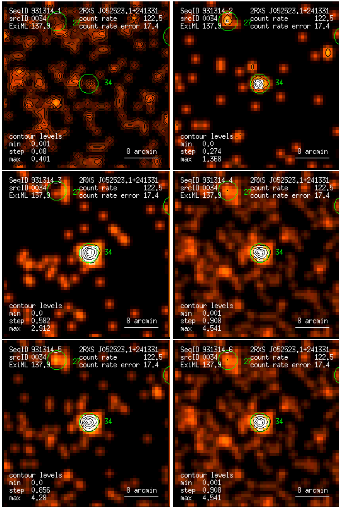
Figure 34: RASS 931314: detection 0034: band rate images, Gaussian filter: (1) PSPC channels 11 – 41, (2) 52 – 90, (3) 91 – 201, (4) 11 – 235, (5) 52 – 201, (6) 11 – 201. Broad band rates in counts/ks. Band rate contour levels in counts/ks/arcmin 2 .
