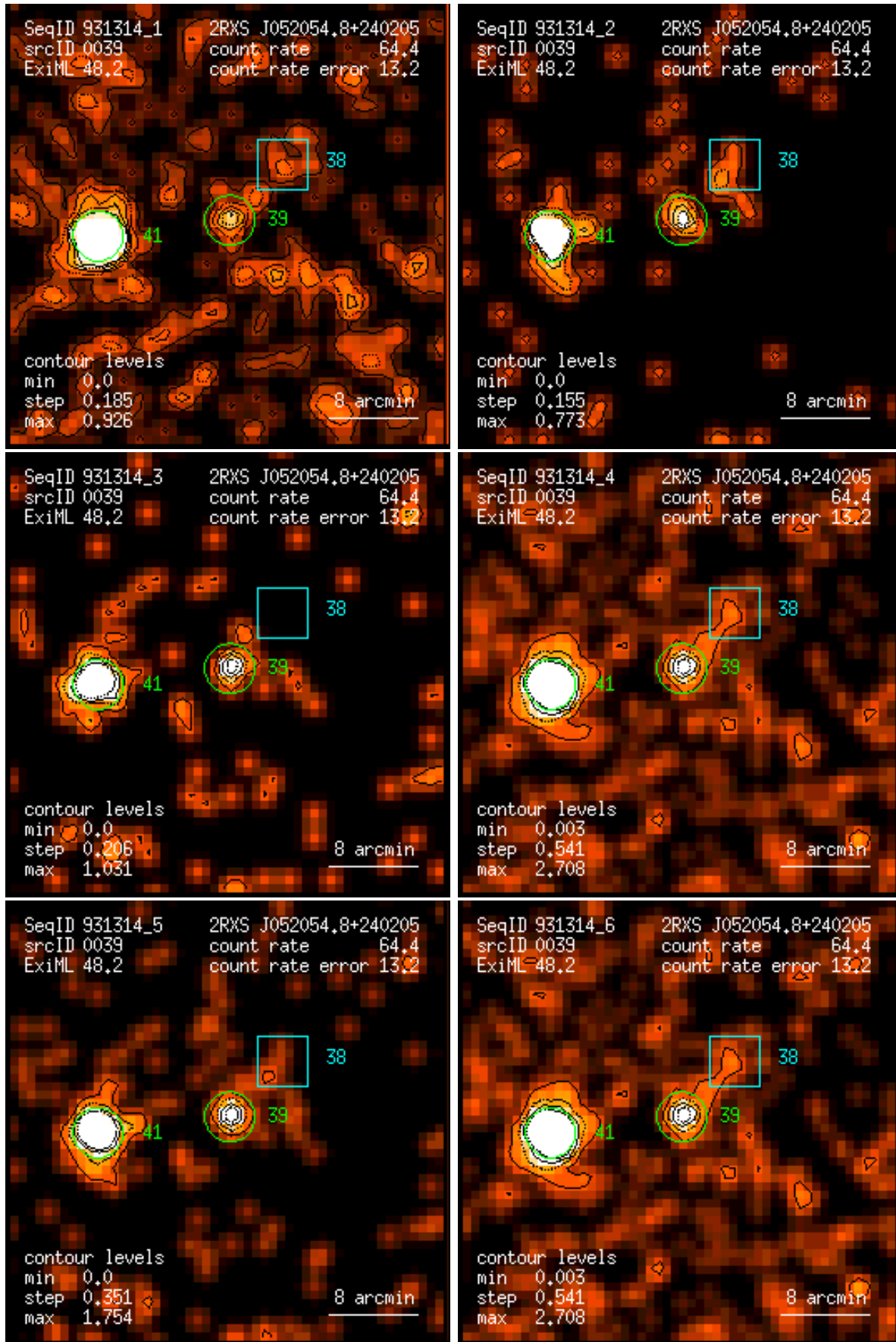
Figure 39: RASS 931314: detection 0039: band rate images, Gaussian filter: (1) PSPC channels 11 – 41, (2) 52 – 90, (3) 91 – 201, (4) 11 – 235, (5) 52 – 201, (6) 11 – 201. Broad band rates in counts/ks. Band rate contour levels in counts/ks/arcmin 2 .
