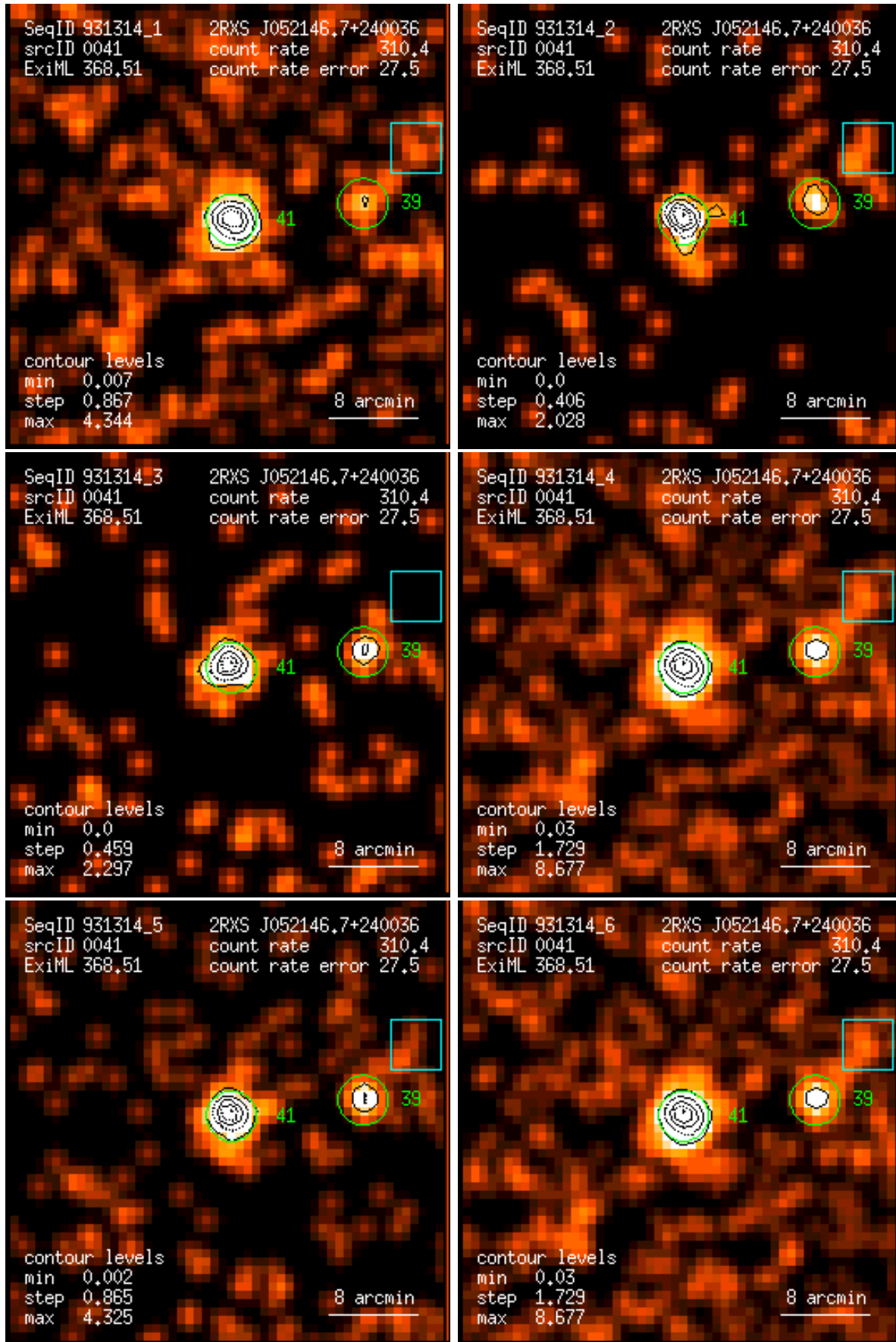
Figure 41: RASS 931314: detection 0041: band rate images, Gaussian filter: (1) PSPC channels 11 – 41, (2) 52 – 90, (3) 91 – 201, (4) 11 – 235, (5) 52 – 201, (6) 11 – 201. Broad band rates in counts/ks. Band rate contour levels in counts/ks/arcmin 2 .
