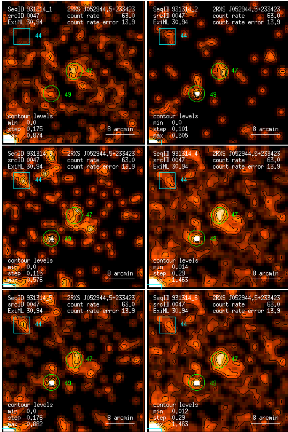
Figure 47: RASS 931314: detection 0047: band rate images, Gaussian filter: (1) PSPC channels 11 – 41, (2) 52 – 90, (3) 91 – 201, (4) 11 – 235, (5) 52 – 201, (6) 11 – 201. Broad band rates in counts/ks. Band rate contour levels in counts/ks/arcmin 2 .
