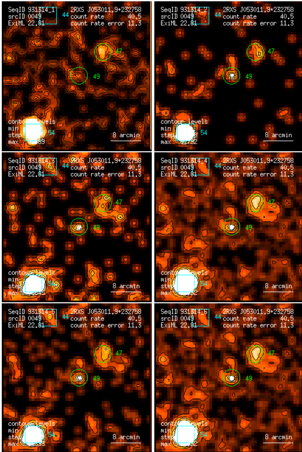
Figure 49: RASS 931314: detection 0049: band rate images, Gaussian filter: (1) PSPC channels 11 – 41, (2) 52 – 90, (3) 91 – 201, (4) 11 – 235, (5) 52 – 201, (6) 11 – 201. Broad band rates in counts/ks. Band rate contour levels in counts/ks/arcmin 2 .
