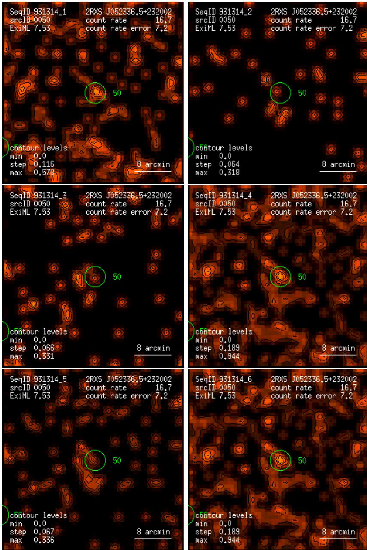
Figure 50: RASS 931314: detection 0050: band rate images, Gaussian filter: (1) PSPC channels 11 – 41, (2) 52 – 90, (3) 91 – 201, (4) 11 – 235, (5) 52 – 201, (6) 11 – 201. Broad band rates in counts/ks. Band rate contour levels in counts/ks/arcmin 2 .
