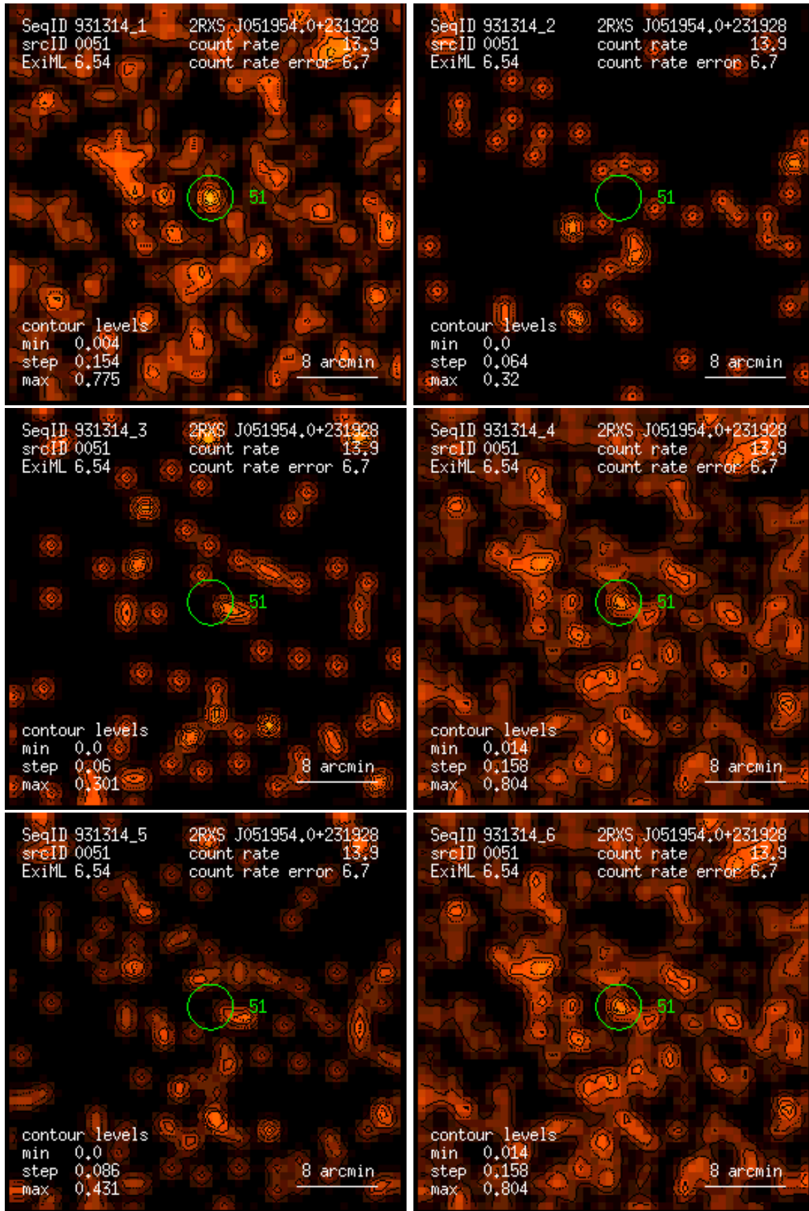
Figure 51: RASS 931314: detection 0051: band rate images, Gaussian filter: (1) PSPC channels 11 – 41, (2) 52 – 90, (3) 91 – 201, (4) 11 – 235, (5) 52 – 201, (6) 11 – 201. Broad band rates in counts/ks. Band rate contour levels in counts/ks/arcmin 2 .
