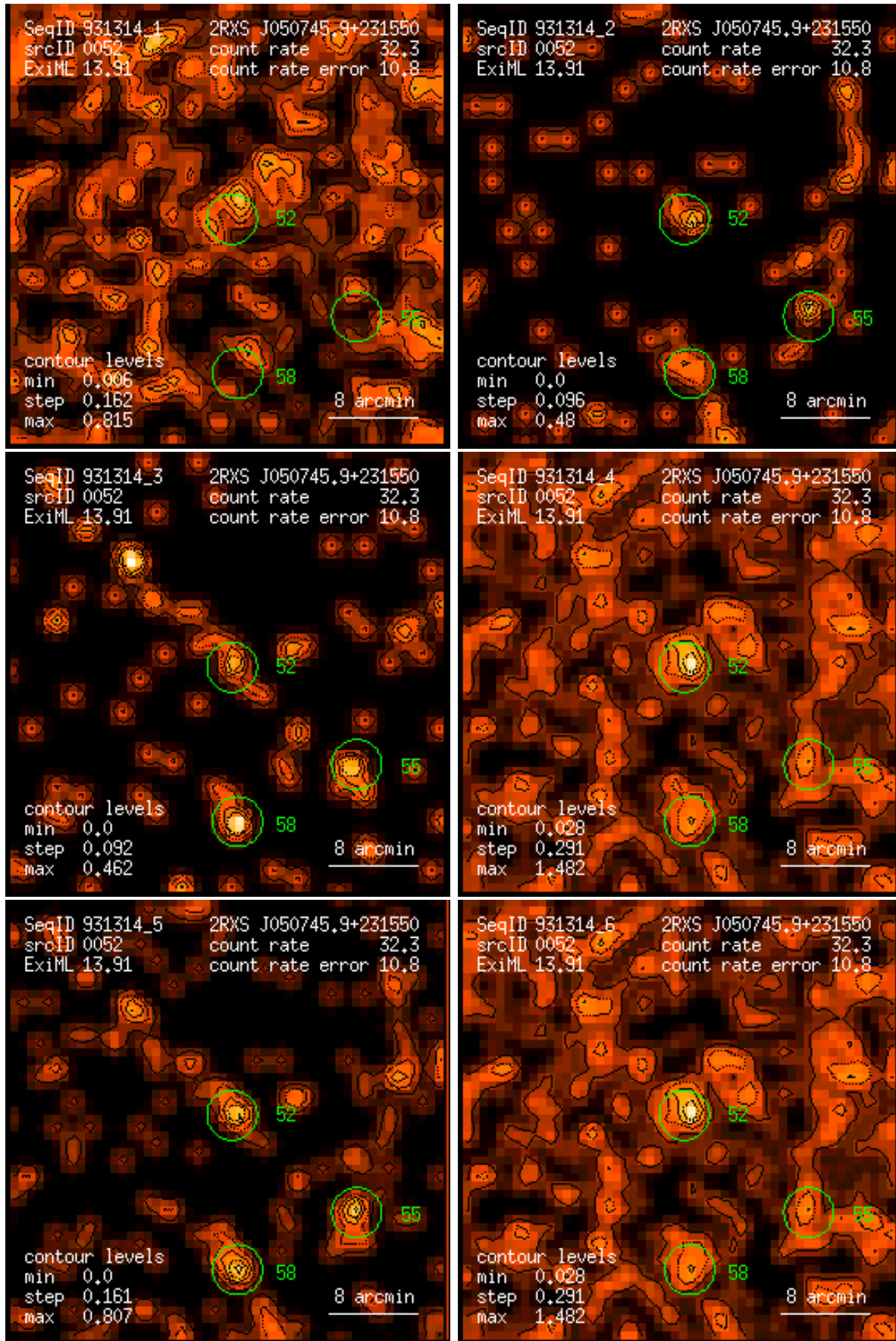
Figure 52: RASS 931314: detection 0052: band rate images, Gaussian filter: (1) PSPC channels 11 – 41, (2) 52 – 90, (3) 91 – 201, (4) 11 – 235, (5) 52 – 201, (6) 11 – 201. Broad band rates in counts/ks. Band rate contour levels in counts/ks/arcmin 2 .
