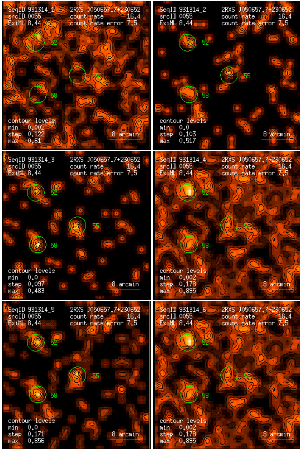
Figure 55: RASS 931314: detection 0055: band rate images, Gaussian filter: (1) PSPC channels 11 – 41, (2) 52 – 90, (3) 91 – 201, (4) 11 – 235, (5) 52 – 201, (6) 11 – 201. Broad band rates in counts/ks. Band rate contour levels in counts/ks/arcmin 2 .
