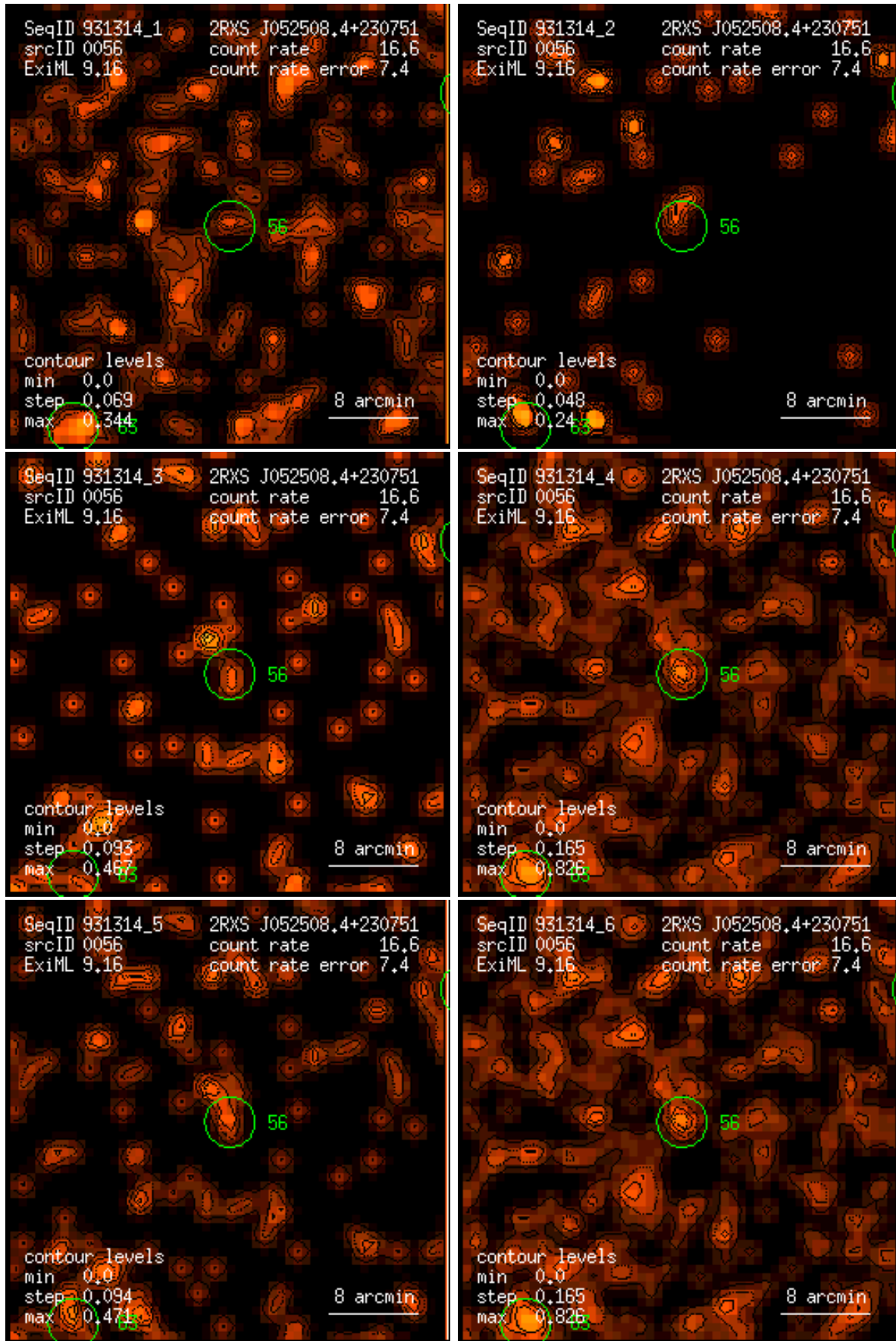
Figure 56: RASS 931314: detection 0056: band rate images, Gaussian filter: (1) PSPC channels 11 – 41, (2) 52 – 90, (3) 91 – 201, (4) 11 – 235, (5) 52 – 201, (6) 11 – 201. Broad band rates in counts/ks. Band rate contour levels in counts/ks/arcmin 2 .
