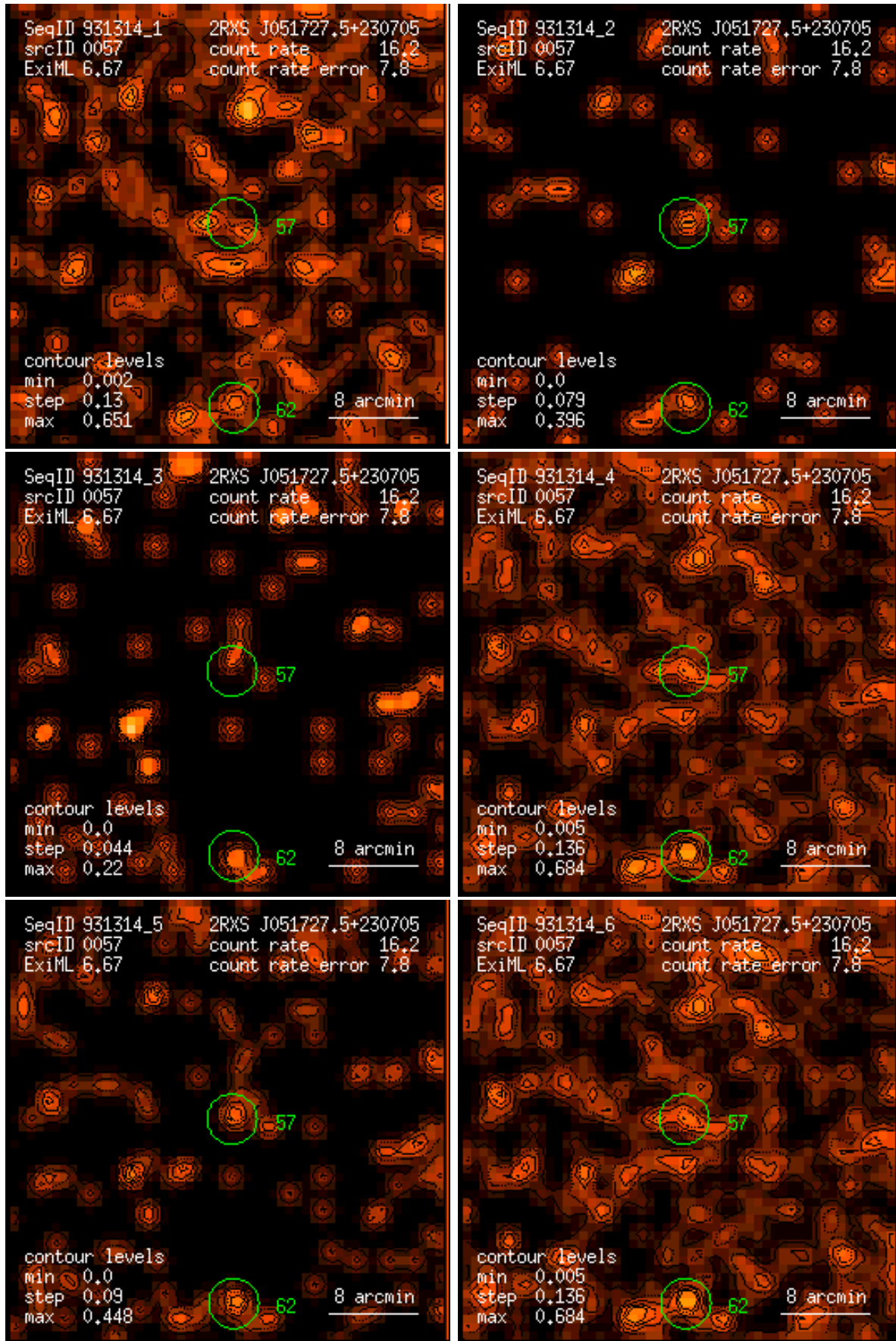
Figure 57: RASS 931314: detection 0057: band rate images, Gaussian filter: (1) PSPC channels 11 – 41, (2) 52 – 90, (3) 91 – 201, (4) 11 – 235, (5) 52 – 201, (6) 11 – 201. Broad band rates in counts/ks. Band rate contour levels in counts/ks/arcmin 2 .
