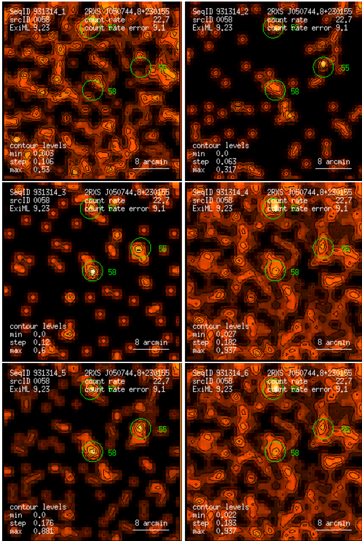
Figure 58: RASS 931314: detection 0058: band rate images, Gaussian filter: (1) PSPC channels 11 – 41, (2) 52 – 90, (3) 91 – 201, (4) 11 – 235, (5) 52 – 201, (6) 11 – 201. Broad band rates in counts/ks. Band rate contour levels in counts/ks/arcmin 2 .
