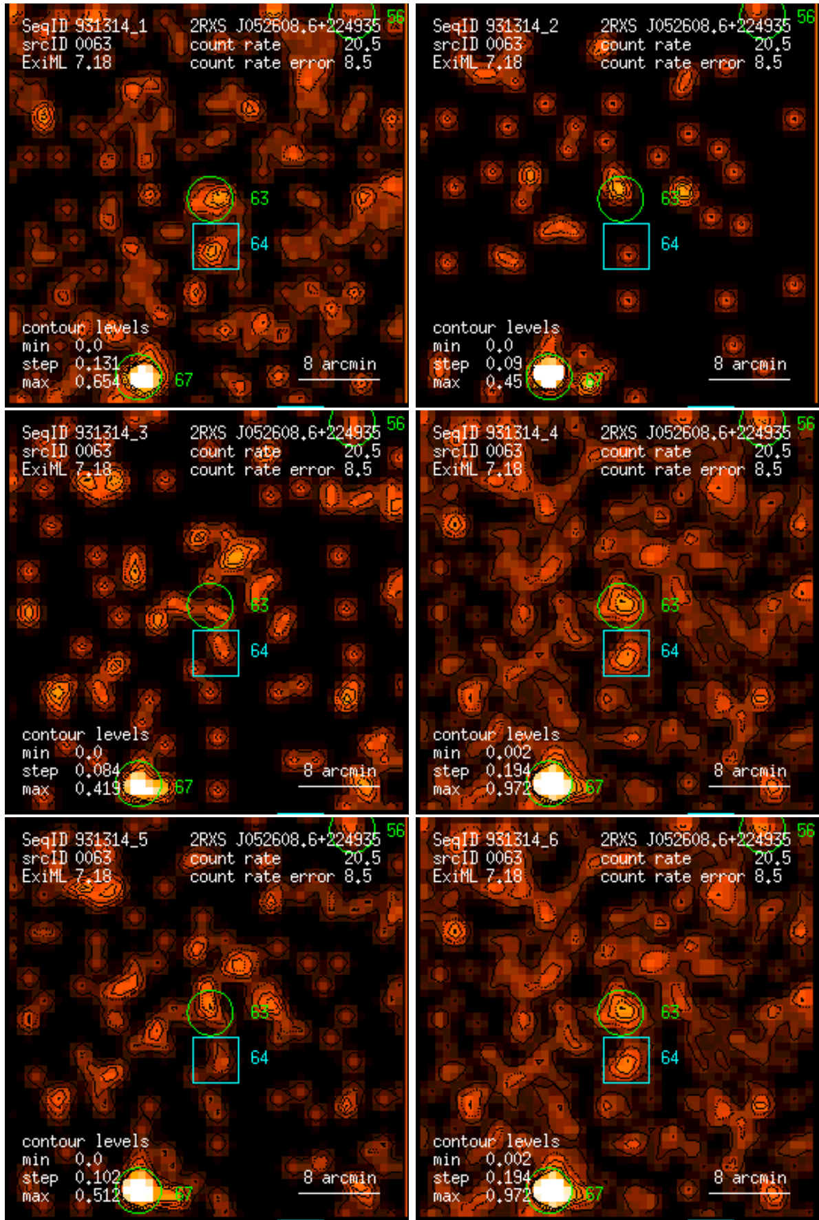
Figure 63: RASS 931314: detection 0063: band rate images, Gaussian filter: (1) PSPC channels 11 – 41, (2) 52 – 90, (3) 91 – 201, (4) 11 – 235, (5) 52 – 201, (6) 11 – 201. Broad band rates in counts/ks. Band rate contour levels in counts/ks/arcmin 2 .
