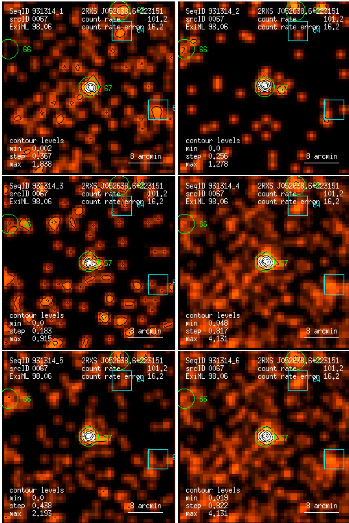
Figure 67: RASS 931314: detection 0067: band rate images, Gaussian filter: (1) PSPC channels 11 – 41, (2) 52 – 90, (3) 91 – 201, (4) 11 – 235, (5) 52 – 201, (6) 11 – 201. Broad band rates in counts/ks. Band rate contour levels in counts/ks/arcmin 2 .
