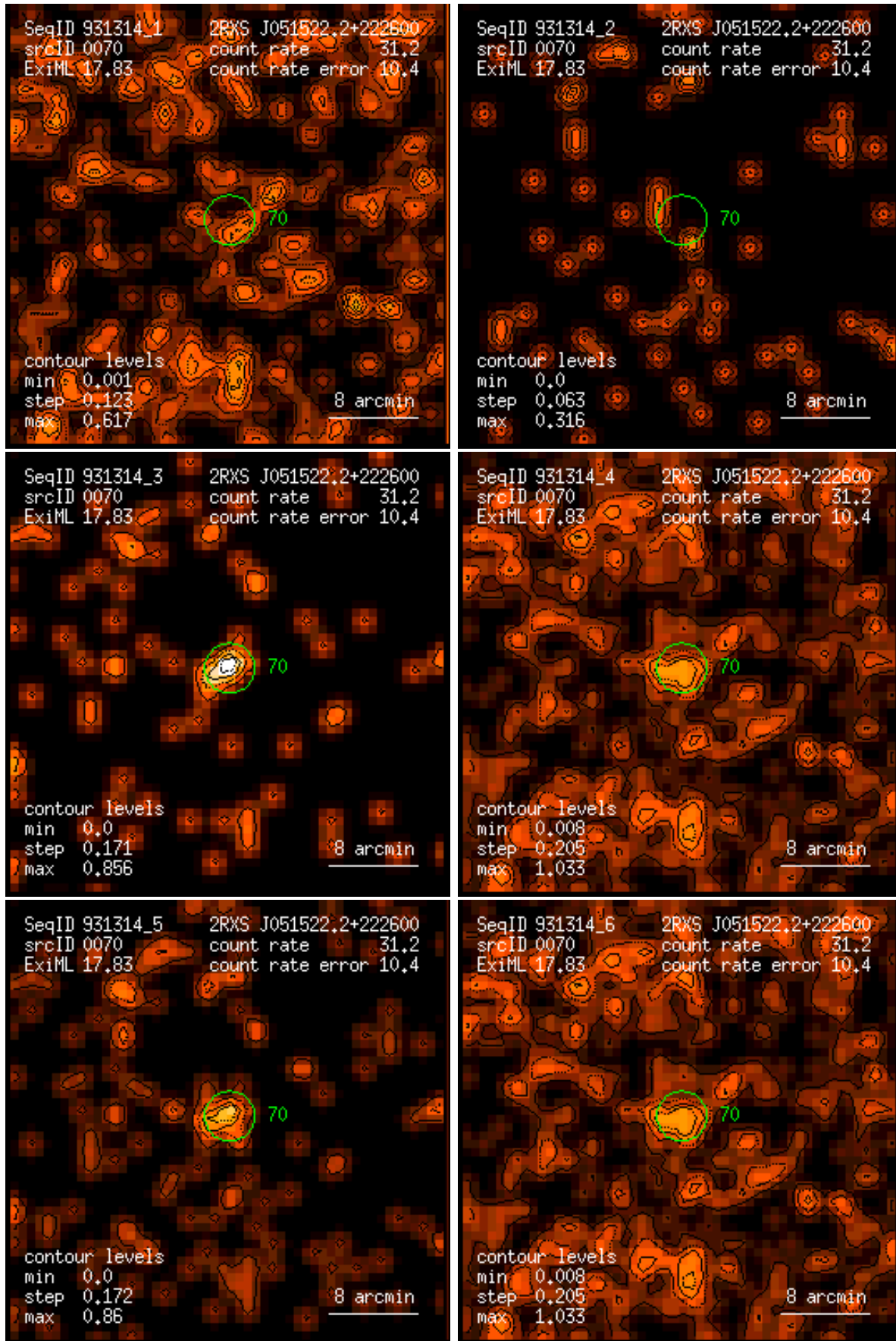
Figure 70: RASS 931314: detection 0070: band rate images, Gaussian filter: (1) PSPC channels 11 – 41, (2) 52 – 90, (3) 91 – 201, (4) 11 – 235, (5) 52 – 201, (6) 11 – 201. Broad band rates in counts/ks. Band rate contour levels in counts/ks/arcmin 2 .
