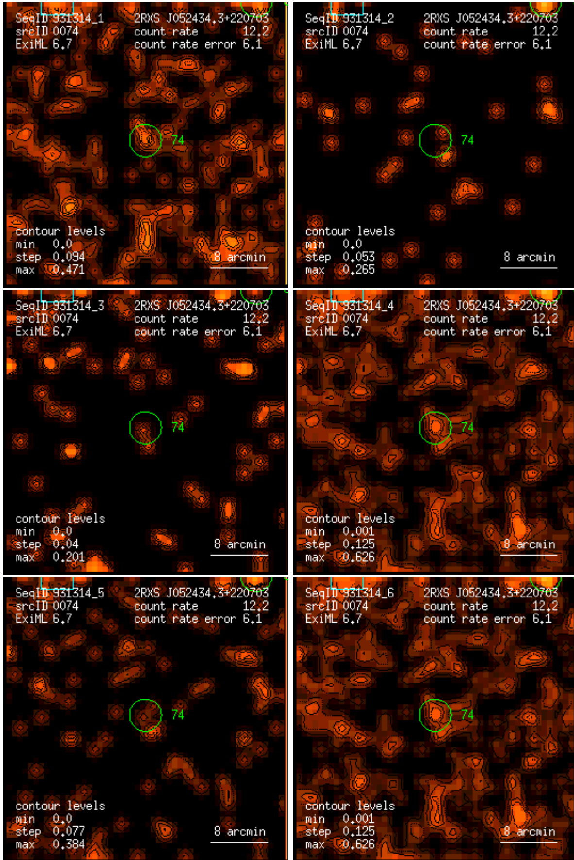
Figure 74: RASS 931314: detection 0074: band rate images, Gaussian filter: (1) PSPC channels 11 – 41, (2) 52 – 90, (3) 91 – 201, (4) 11 – 235, (5) 52 – 201, (6) 11 – 201. Broad band rates in counts/ks. Band rate contour levels in counts/ks/arcmin 2 .
