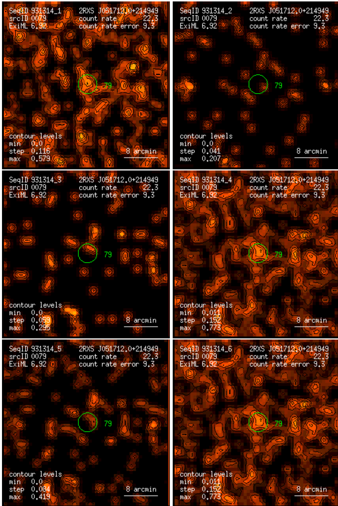
Figure 79: RASS 931314: detection 0079: band rate images, Gaussian filter: (1) PSPC channels 11 – 41, (2) 52 – 90, (3) 91 – 201, (4) 11 – 235, (5) 52 – 201, (6) 11 – 201. Broad band rates in counts/ks. Band rate contour levels in counts/ks/arcmin 2 .
