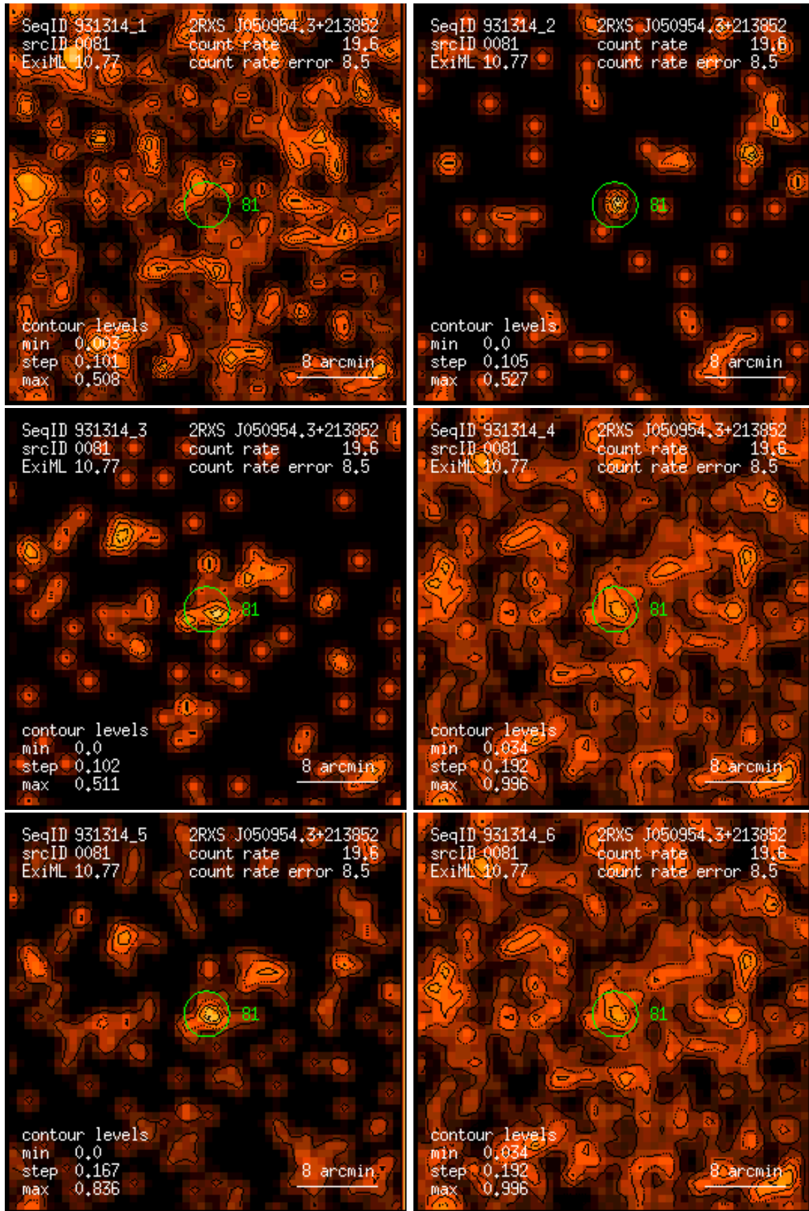
Figure 81: RASS 931314: detection 0081: band rate images, Gaussian filter: (1) PSPC channels 11 – 41, (2) 52 – 90, (3) 91 – 201, (4) 11 – 235, (5) 52 – 201, (6) 11 – 201. Broad band rates in counts/ks. Band rate contour levels in counts/ks/arcmin 2 .
