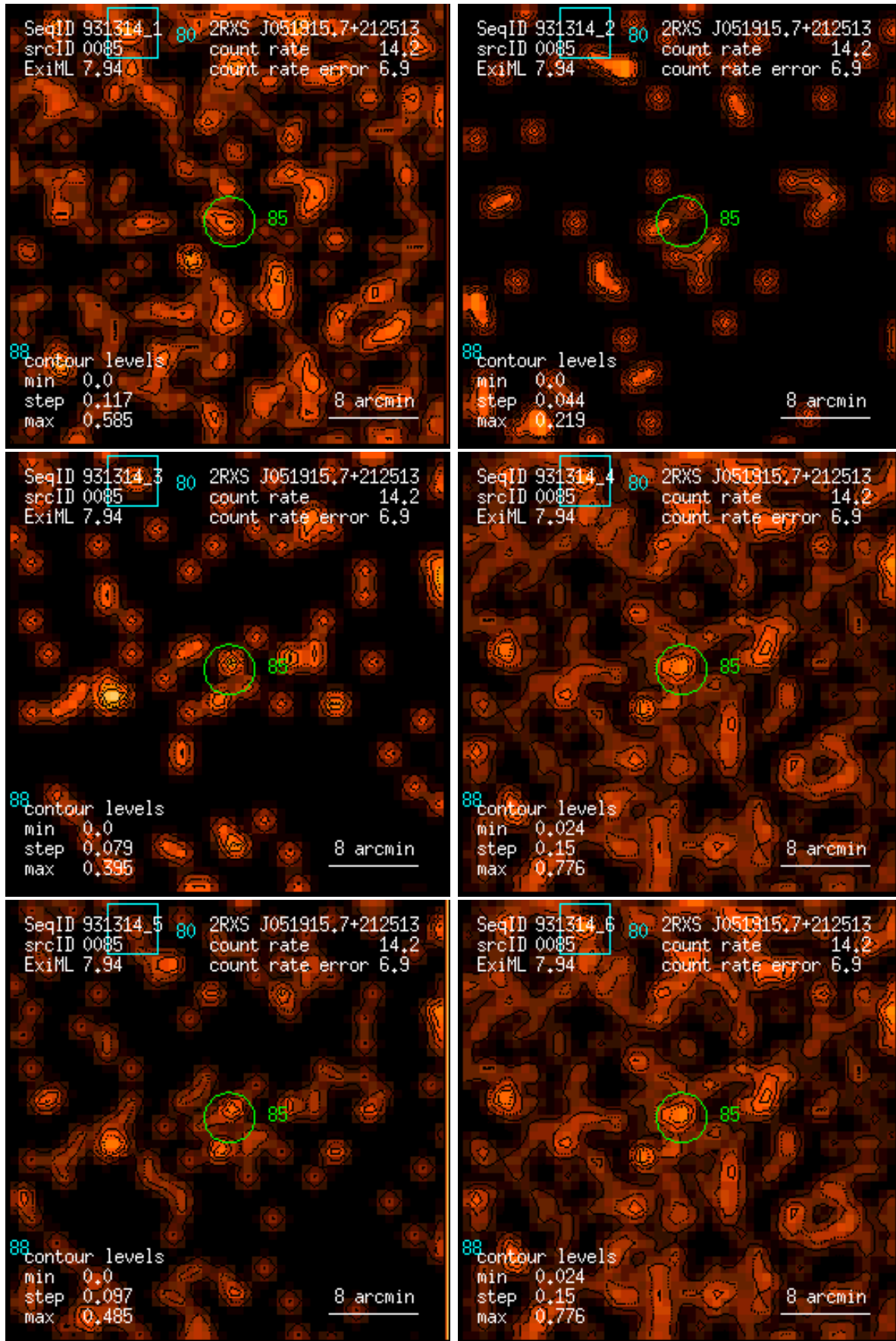
Figure 85: RASS 931314: detection 0085: band rate images, Gaussian filter: (1) PSPC channels 11 – 41, (2) 52 – 90, (3) 91 – 201, (4) 11 – 235, (5) 52 – 201, (6) 11 – 201. Broad band rates in counts/ks. Band rate contour levels in counts/ks/arcmin 2 .
