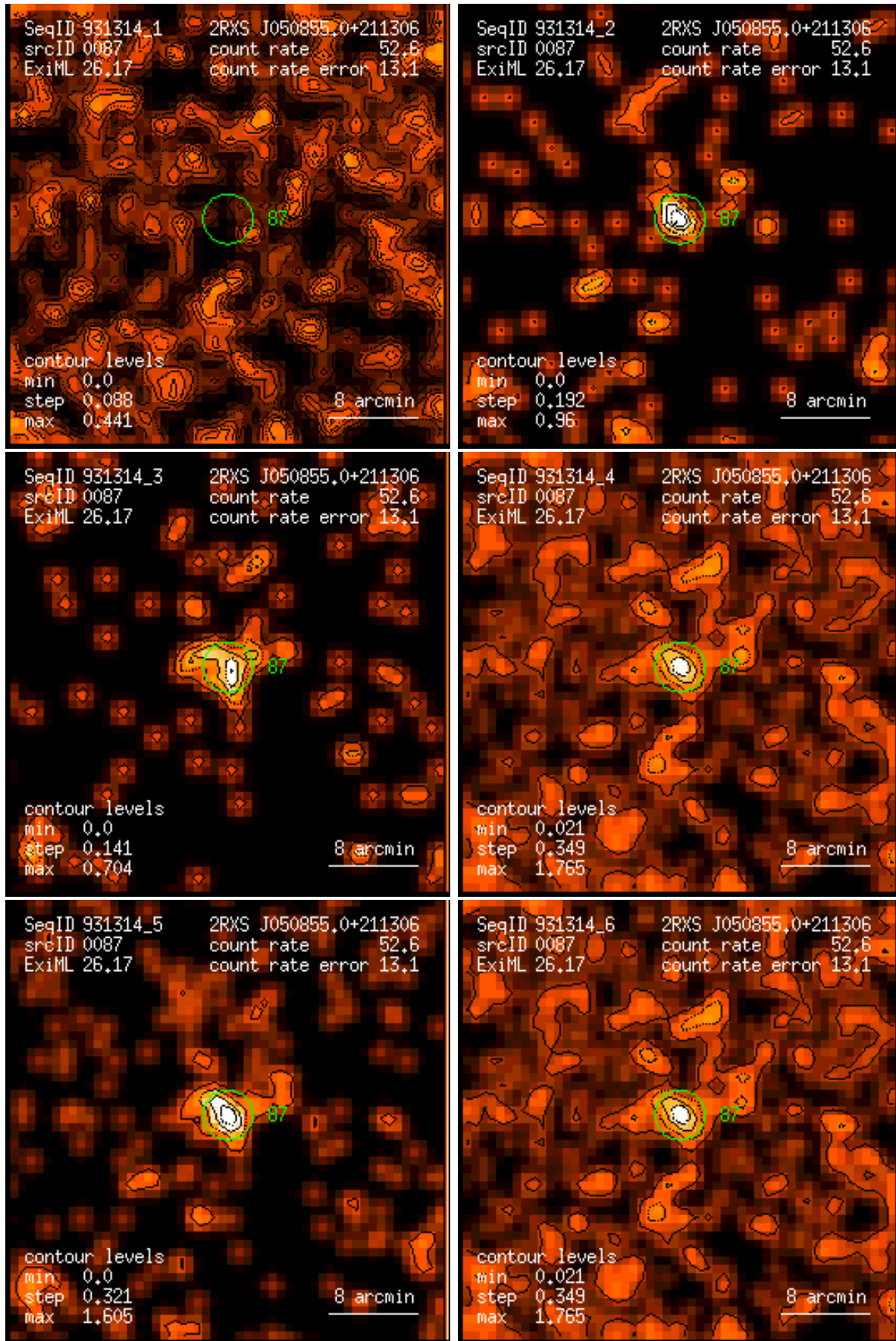
Figure 87: RASS 931314: detection 0087: band rate images, Gaussian filter: (1) PSPC channels 11 – 41, (2) 52 – 90, (3) 91 – 201, (4) 11 – 235, (5) 52 – 201, (6) 11 – 201. Broad band rates in counts/ks. Band rate contour levels in counts/ks/arcmin 2 .
