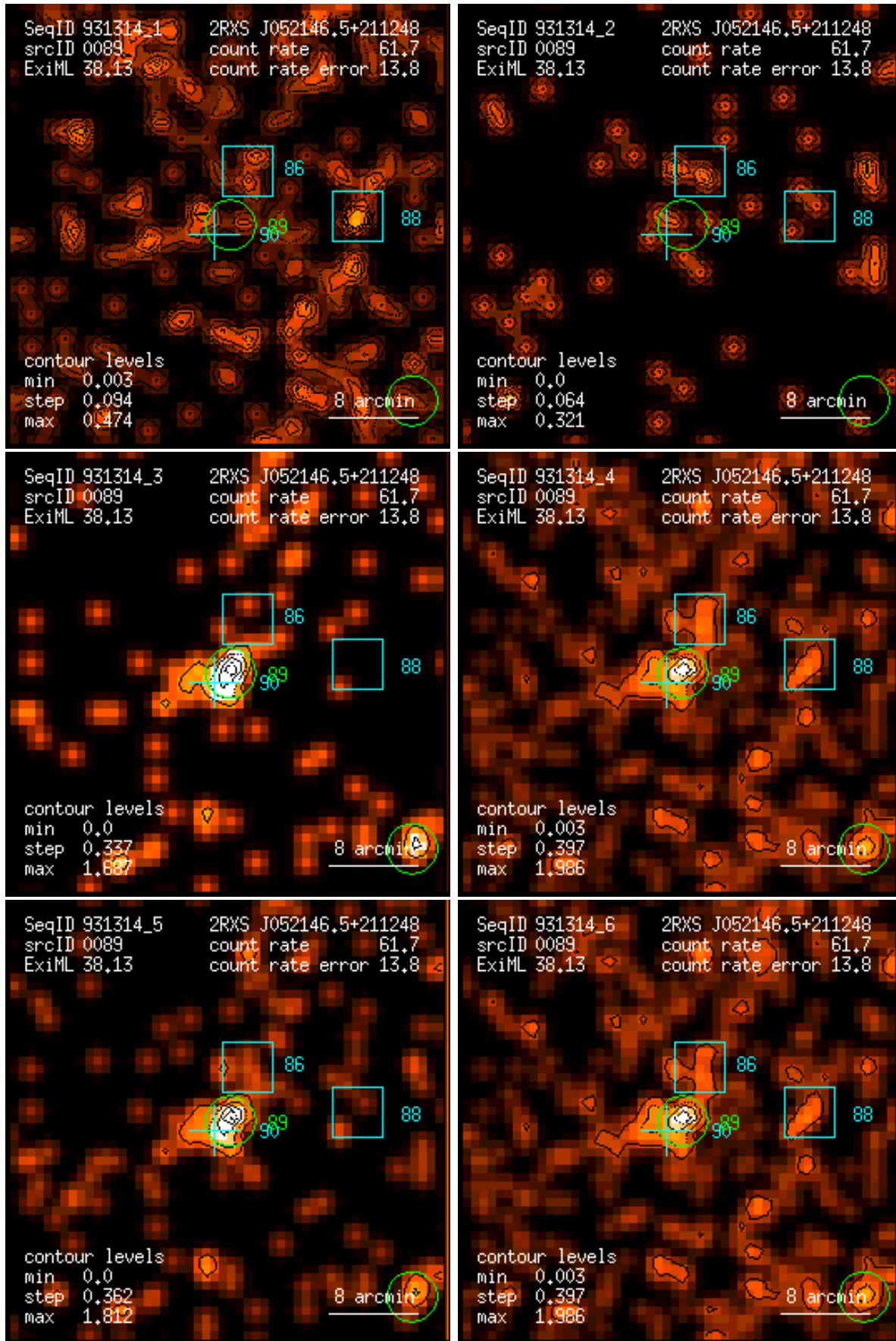
Figure 89: RASS 931314: detection 0089: band rate images, Gaussian filter: (1) PSPC channels 11 – 41, (2) 52 – 90, (3) 91 – 201, (4) 11 – 235, (5) 52 – 201, (6) 11 – 201. Broad band rates in counts/ks. Band rate contour levels in counts/ks/arcmin 2 .
