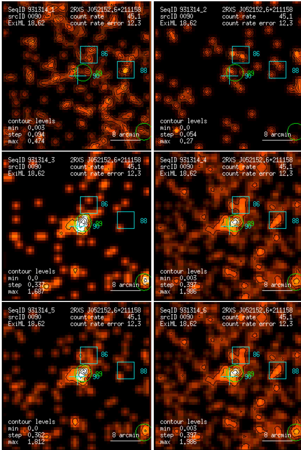
Figure 90: RASS 931314: detection 0090: band rate images, Gaussian filter: (1) PSPC channels 11 – 41, (2) 52 – 90, (3) 91 – 201, (4) 11 – 235, (5) 52 – 201, (6) 11 – 201. Broad band rates in counts/ks. Band rate contour levels in counts/ks/arcmin 2 .
