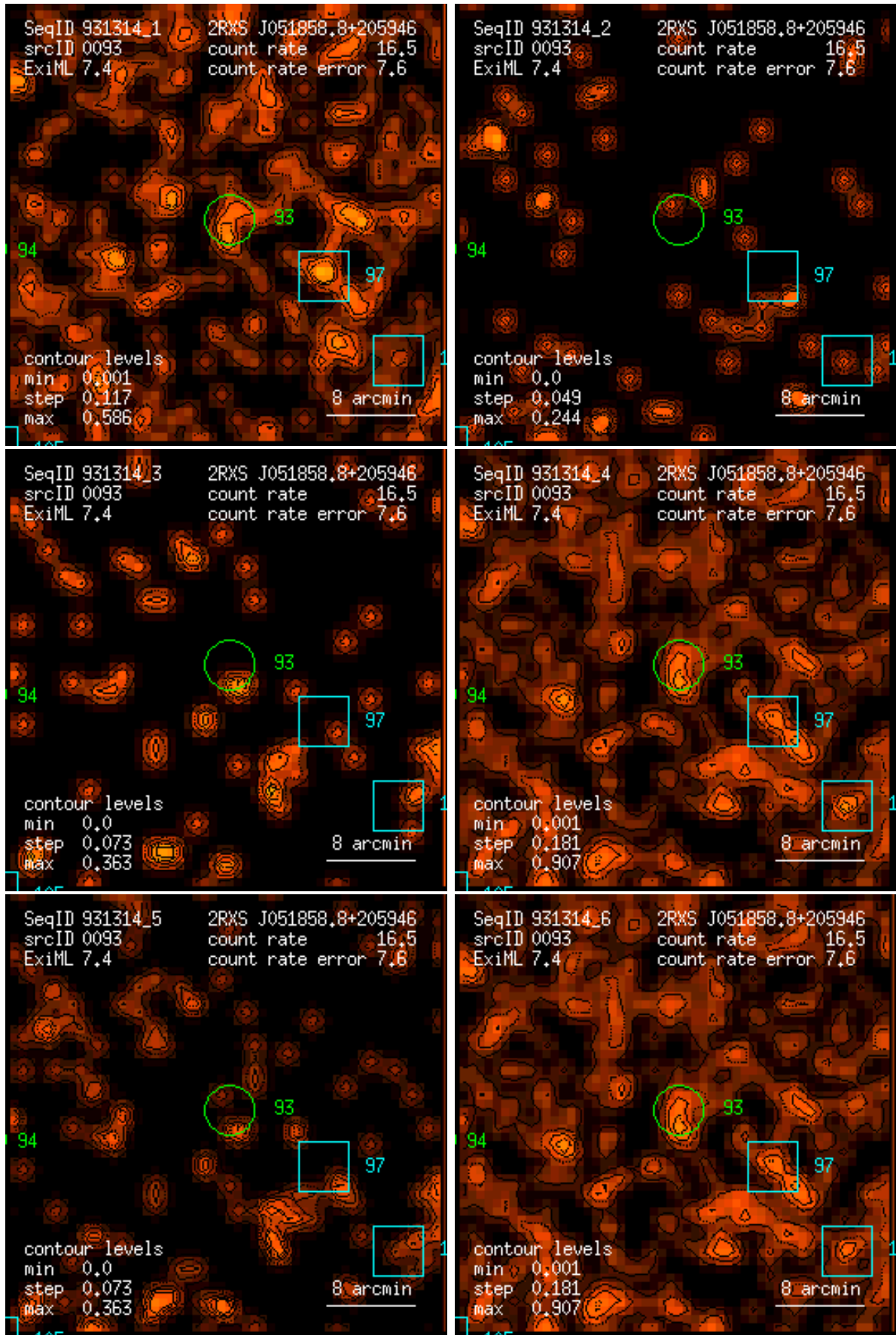
Figure 93: RASS 931314: detection 0093: band rate images, Gaussian filter: (1) PSPC channels 11 – 41, (2) 52 – 90, (3) 91 – 201, (4) 11 – 235, (5) 52 – 201, (6) 11 – 201. Broad band rates in counts/ks. Band rate contour levels in counts/ks/arcmin 2 .
