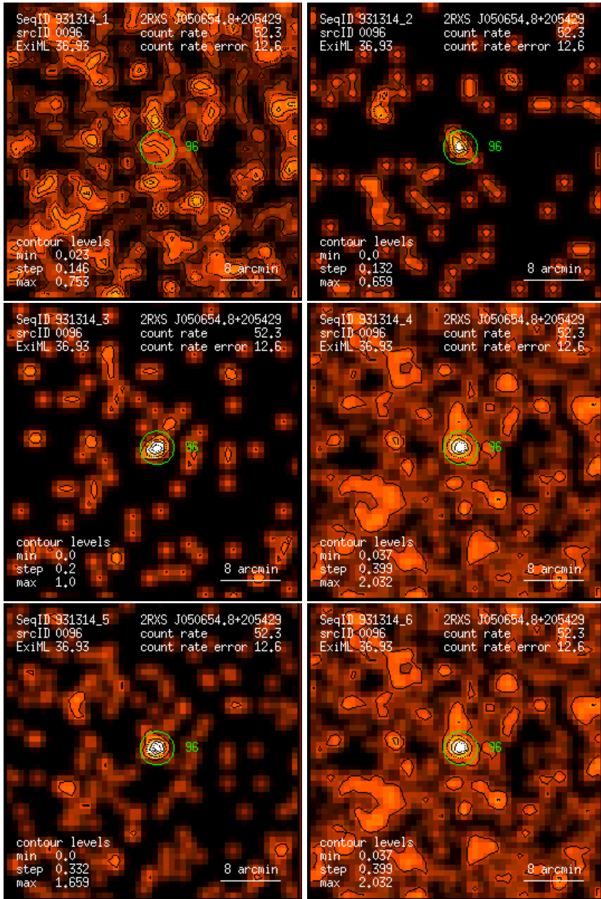
Figure 96: RASS 931314: detection 0096: band rate images, Gaussian filter: (1) PSPC channels 11 – 41, (2) 52 – 90, (3) 91 – 201, (4) 11 – 235, (5) 52 – 201, (6) 11 – 201. Broad band rates in counts/ks. Band rate contour levels in counts/ks/arcmin 2 .
