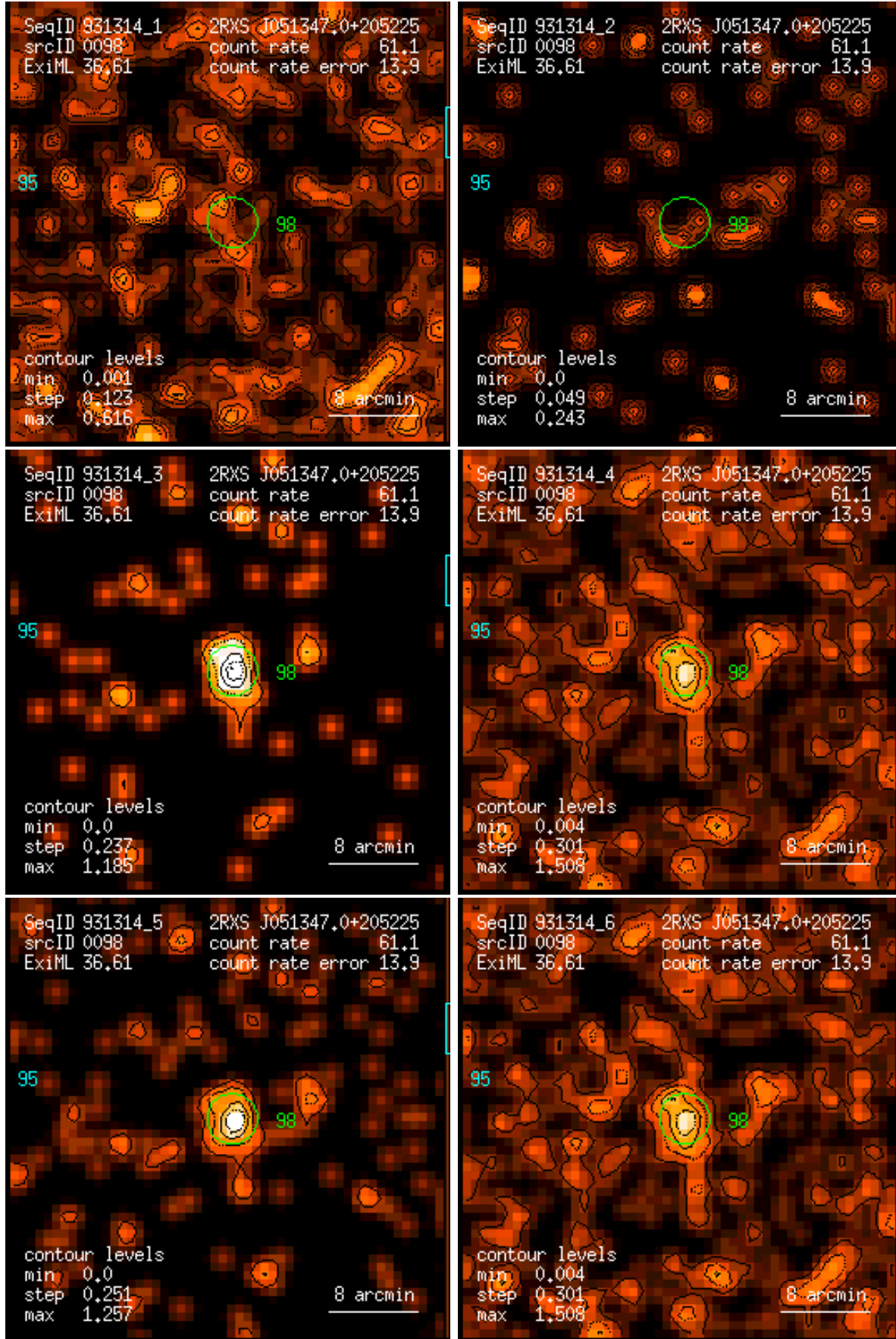
Figure 98: RASS 931314: detection 0098: band rate images, Gaussian filter: (1) PSPC channels 11 – 41, (2) 52 – 90, (3) 91 – 201, (4) 11 – 235, (5) 52 – 201, (6) 11 – 201. Broad band rates in counts/ks. Band rate contour levels in counts/ks/arcmin 2 .
