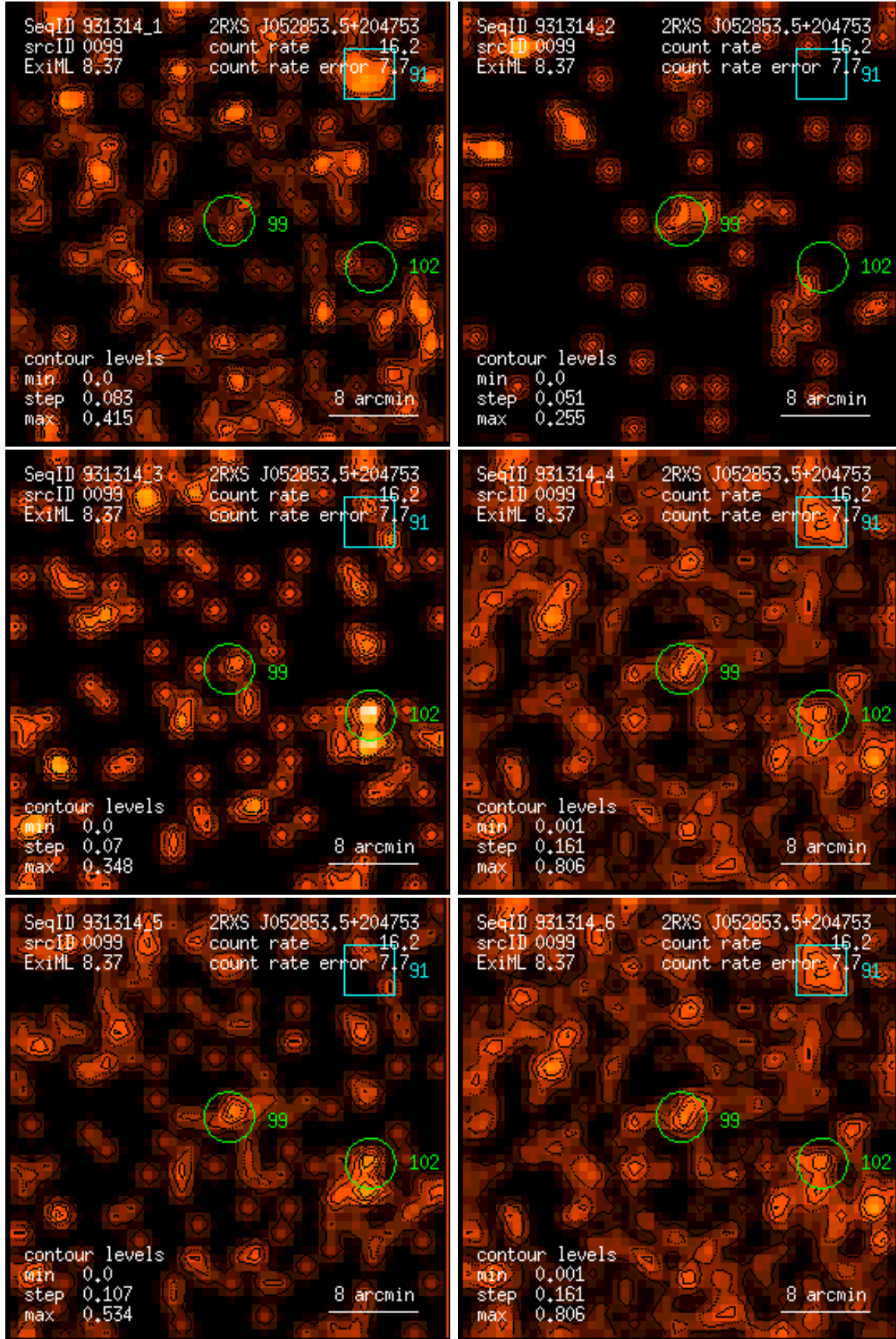
Figure 99: RASS 931314: detection 0099: band rate images, Gaussian filter: (1) PSPC channels 11 – 41, (2) 52 – 90, (3) 91 – 201, (4) 11 – 235, (5) 52 – 201, (6) 11 – 201. Broad band rates in counts/ks. Band rate contour levels in counts/ks/arcmin 2 .
