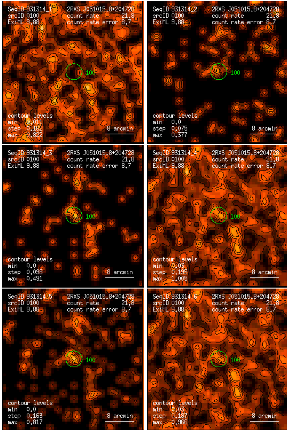
Figure 100: RASS 931314: detection 0100: band rate images, Gaussian filter: (1) PSPC channels 11 – 41, (2) 52 – 90, (3) 91 – 201, (4) 11 – 235, (5) 52 – 201, (6) 11 – 201. Broad band rates in counts/ks. Band rate contour levels in counts/ks/arcmin 2 .
