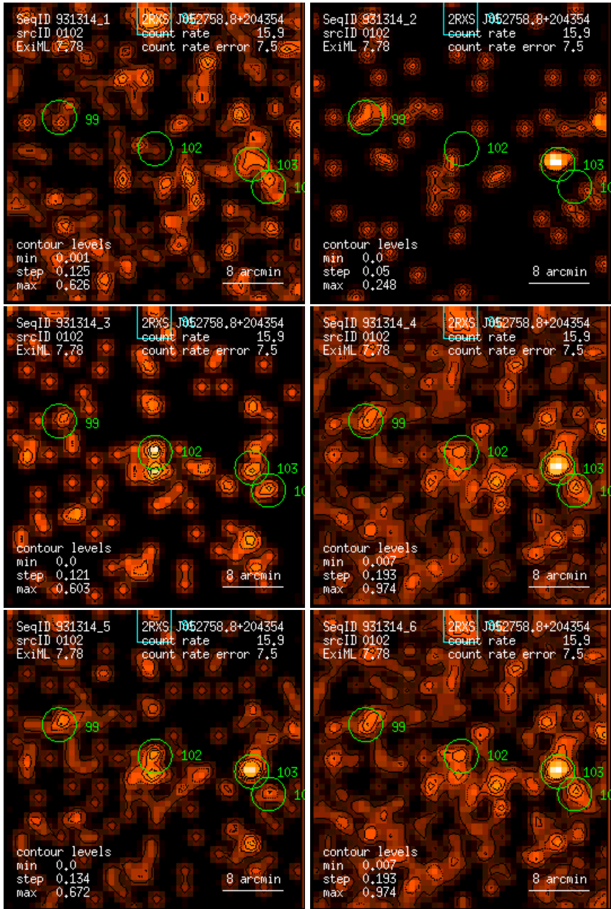
Figure 102: RASS 931314: detection 0102: band rate images, Gaussian filter: (1) PSPC channels 11 – 41, (2) 52 – 90, (3) 91 – 201, (4) 11 – 235, (5) 52 – 201, (6) 11 – 201. Broad band rates in counts/ks. Band rate contour levels in counts/ks/arcmin 2 .
