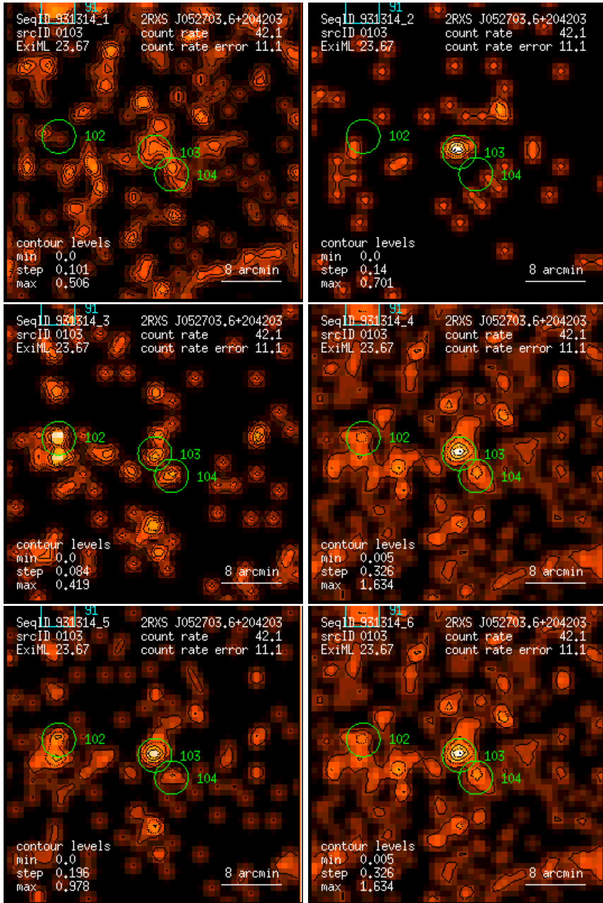
Figure 103: RASS 931314: detection 0103: band rate images, Gaussian filter: (1) PSPC channels 11 – 41, (2) 52 – 90, (3) 91 – 201, (4) 11 – 235, (5) 52 – 201, (6) 11 – 201. Broad band rates in counts/ks. Band rate contour levels in counts/ks/arcmin 2 .
