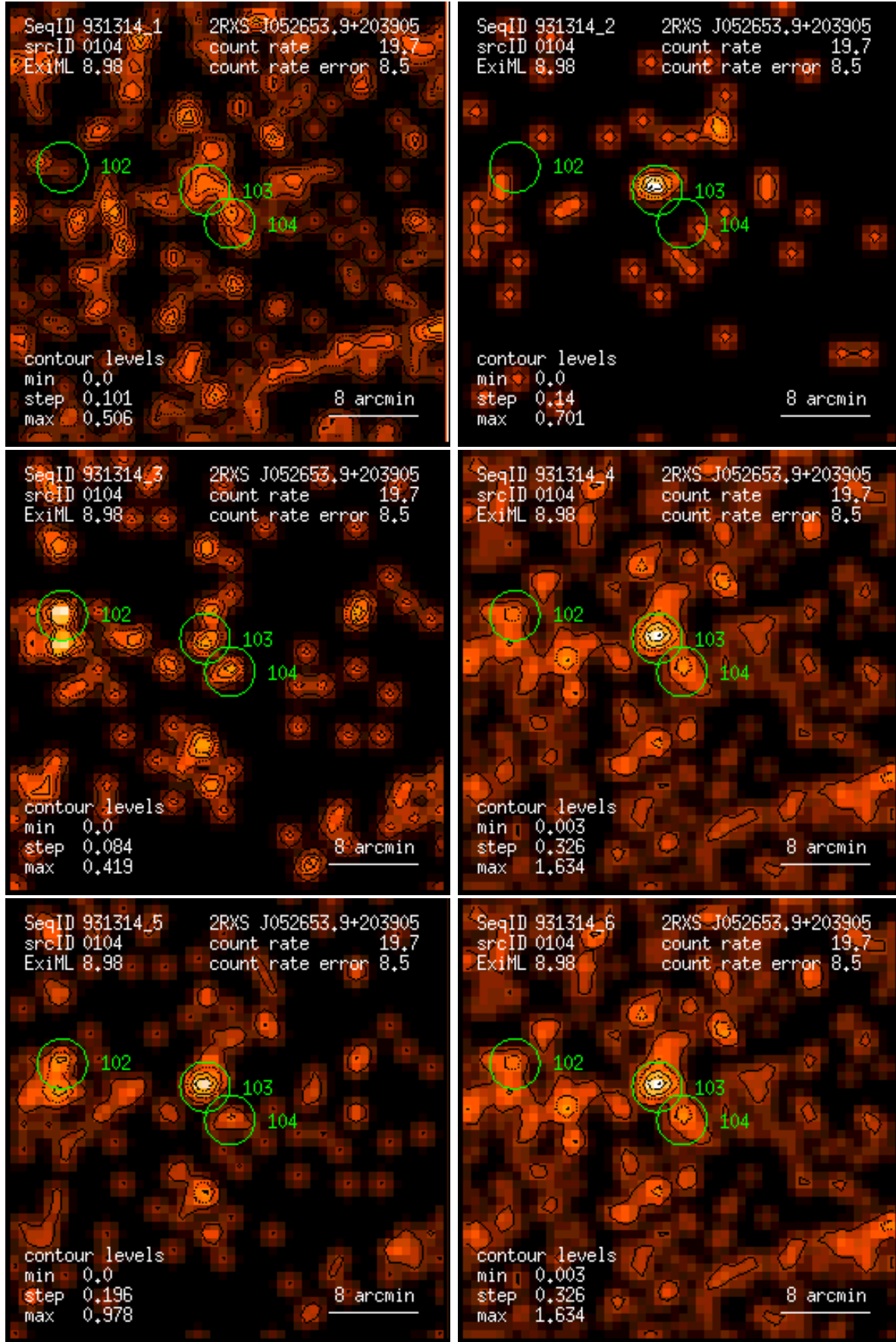
Figure 104: RASS 931314: detection 0104: band rate images, Gaussian filter: (1) PSPC channels 11 – 41, (2) 52 – 90, (3) 91 – 201, (4) 11 – 235, (5) 52 – 201, (6) 11 – 201. Broad band rates in counts/ks. Band rate contour levels in counts/ks/arcmin 2 .
