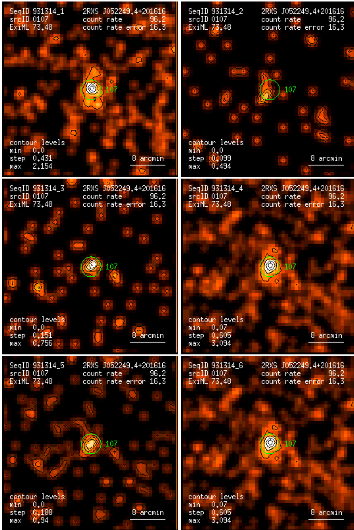
Figure 107: RASS 931314: detection 0107: band rate images, Gaussian filter: (1) PSPC channels 11 – 41, (2) 52 – 90, (3) 91 – 201, (4) 11 – 235, (5) 52 – 201, (6) 11 – 201. Broad band rates in counts/ks. Band rate contour levels in counts/ks/arcmin 2 .
