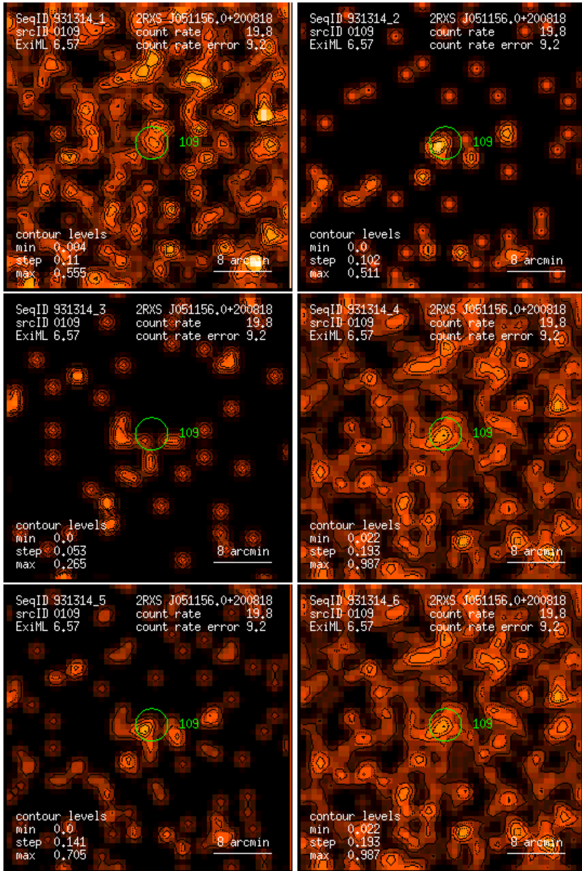
Figure 109: RASS 931314: detection 0109: band rate images, Gaussian filter: (1) PSPC channels 11 – 41, (2) 52 – 90, (3) 91 – 201, (4) 11 – 235, (5) 52 – 201, (6) 11 – 201. Broad band rates in counts/ks. Band rate contour levels in counts/ks/arcmin 2 .
