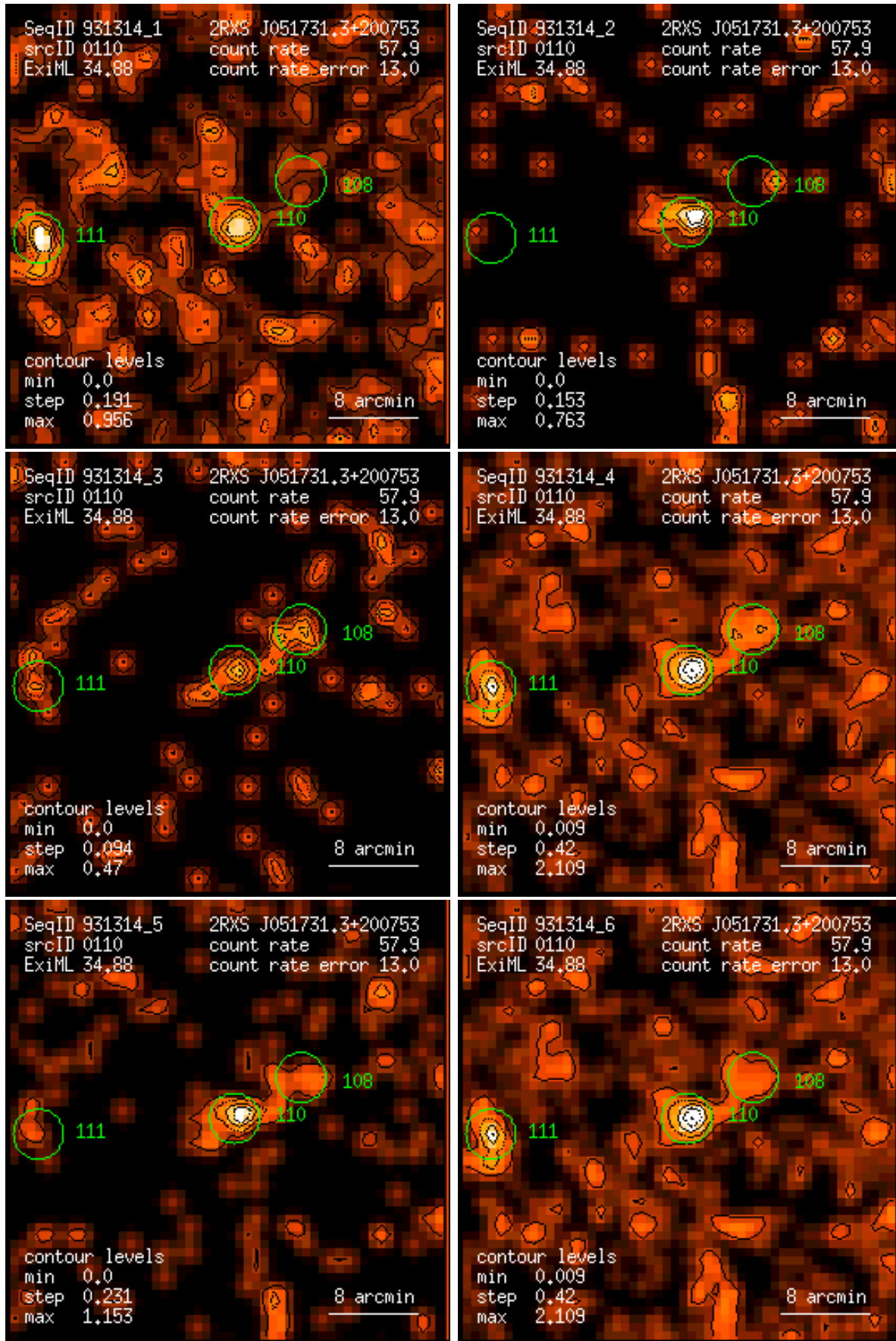
Figure 110: RASS 931314: detection 0110: band rate images, Gaussian filter: (1) PSPC channels 11 – 41, (2) 52 – 90, (3) 91 – 201, (4) 11 – 235, (5) 52 – 201, (6) 11 – 201. Broad band rates in counts/ks. Band rate contour levels in counts/ks/arcmin 2 .
