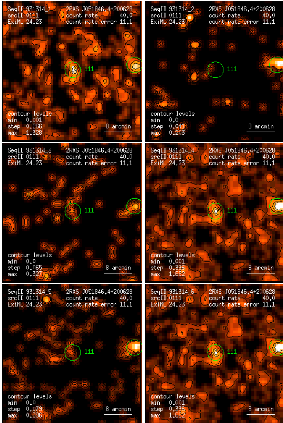
Figure 111: RASS 931314: detection 0111: band rate images, Gaussian filter: (1) PSPC channels 11 – 41, (2) 52 – 90, (3) 91 – 201, (4) 11 – 235, (5) 52 – 201, (6) 11 – 201. Broad band rates in counts/ks. Band rate contour levels in counts/ks/arcmin 2 .
