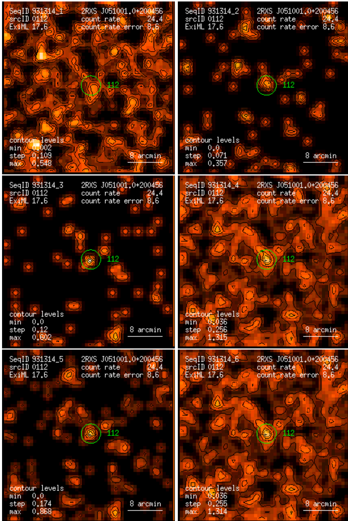
Figure 112: RASS 931314: detection 0112: band rate images, Gaussian filter: (1) PSPC channels 11 – 41, (2) 52 – 90, (3) 91 – 201, (4) 11 – 235, (5) 52 – 201, (6) 11 – 201. Broad band rates in counts/ks. Band rate contour levels in counts/ks/arcmin 2 .
